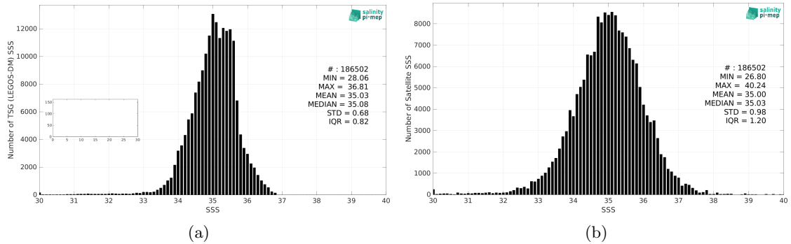
Figure 2: Histograms of SSS from TSG (LEGOS-DM) (a) and SMOS SSS L2Q v331 - 0.25 Deg (CATDS-CPDC) (b) considering all match-up pairs per bins of 0.1 over the Pacific Ocean Pi-MEP region and for the full satellite product period.
