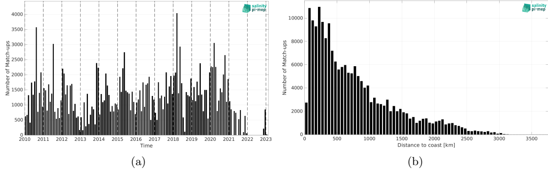
Figure 1: Number of match-ups between TSG (LEGOS-DM) and SMOS SSS L2Q v331 - 0.25 Deg (CATDS-CPDC) SSS as a function of time (a) and as function of the distance to coast (b) over the Pacific Ocean Pi-MEP region and for the full satellite product period.
