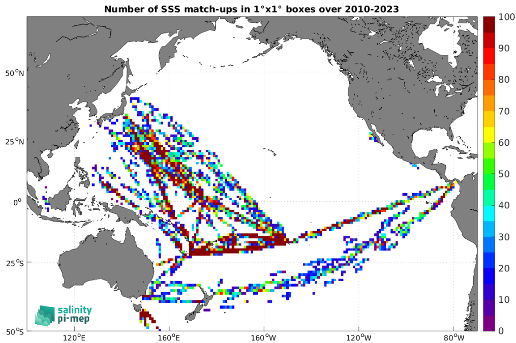
Figure 4: Number of SSS match-ups between TSG (LEGOS-DM) SSS and the SMOS SSS L2Q v331 - 0.25 Deg (CATDS-CPDC) SSS product for the Pacific Ocean Pi-MEP region over 1^\circ \times 1^\circ boxes and for the full satellite product period.
