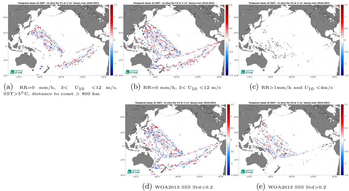
Figure 12: Temporal mean gridded over spatial boxes of size 1^\circ \times 1^\circ of \Delta SSS (SMOS SSS L2Q v331 - 0.25 Deg (CATDS-CPDC) - TSG (LEGOS-DM)) for 5 different subdatasets corresponding to:RR=0 mm/h, 3 < U_{10} < 12 m/s, SST >5^\circ C, distance to coast > 800 km (a), RR=0 mm/h, 3 < U_{10} < 12 m/s (b), RR >1 mm/h and U_{10} < 4 m/s (c), WOA2013 SSS Std <0.2 (d), WOA2013 SSS Std >0.2 (e).
