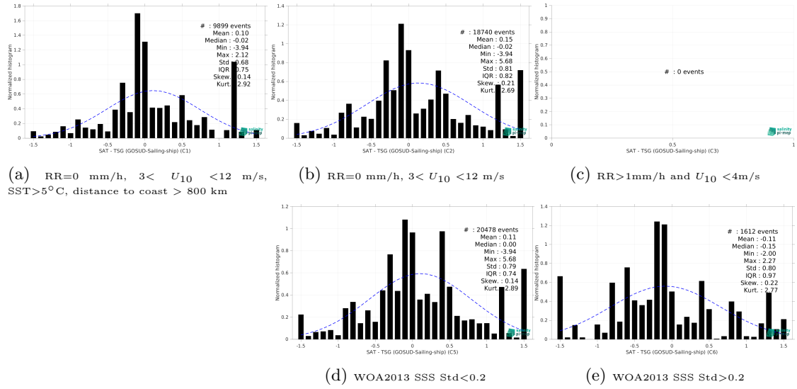
Figure 13: Normalized histogram of \Delta SSS (SMOS SSS L2Q v331 - 0.25 Deg (CATDS-CPDC) - TSG (GOSUD-Sailing-ship)) for 5 different subdatasets corresponding to: RR=0 mm/h, 3 < U_{10} < 12 m/s, SST > 5°C, distance to coast > 800 km (a), RR=0 mm/h, 3 < U_{10} < 12 m/s (b), RR > 1mm/h and U_{10} < 4 m/s (c), WOA2013 SSS Std < 0.2 (d), WOA2013 SSS Std > 0.2 (e).
