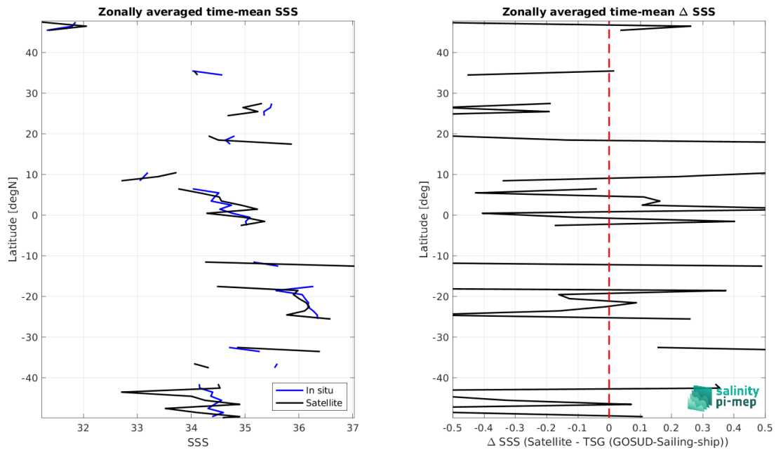
Figure 8: Left panel: Zonal mean SSS from SMOS SSS L2Q v331 - 0.25 Deg (CATDS-CPDC) satellite product (black) and from TSG (GOSUD-Sailing-ship) (blue). Right panel: Zonal mean of \Delta SSS (Satellite - TSG (GOSUD-Sailing-ship)) for all the collected Pi-MEP match-up pairs estimated over the full satellite product period.
