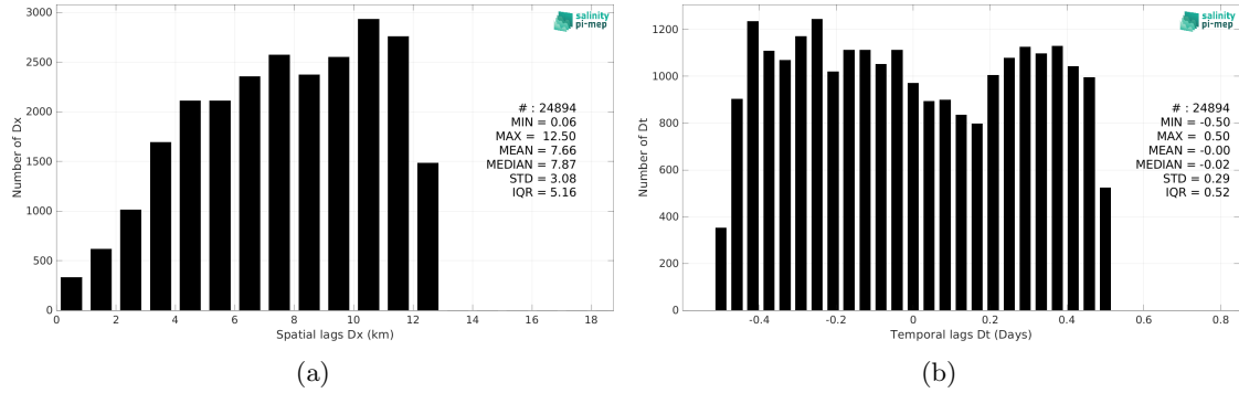
Figure 5: Histograms of the spatial (a) and temporal (b) lags between the location/time of the TSG (GOSUD-Sailing-ship) measurement and the date of the corresponding SMOS SSS L2Q v331 - 0.25 Deg (CATDS-CPDC) SSS pixel.
