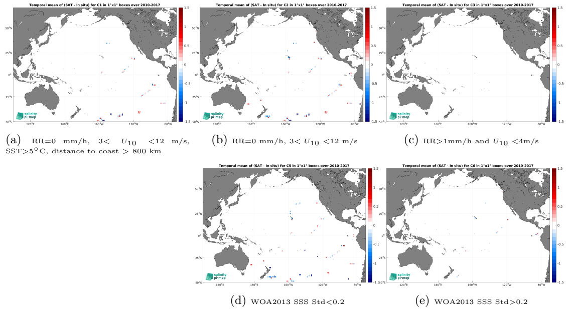
Figure 12: Temporal mean gridded over spatial boxes of size 1^\circ \times 1^\circ of \Delta SSS (SMOS SSS L2Q v331 - 0.25 Deg (CATDS-CPDC) - TSG (GOSUD-Sailing-ship)) for 5 different subdatasets corresponding to:RR=0 mm/h, 3 < U_{10} < 12 m/s, SST >5^\circ C, distance to coast > 800 km (a), RR=0 mm/h, 3 < U_{10} < 12 m/s (b), RR >1 mm/h and U_{10} < 4 m/s (c), WOA2013 SSS Std <0.2 (d), WOA2013 SSS Std >0.2 (e).
