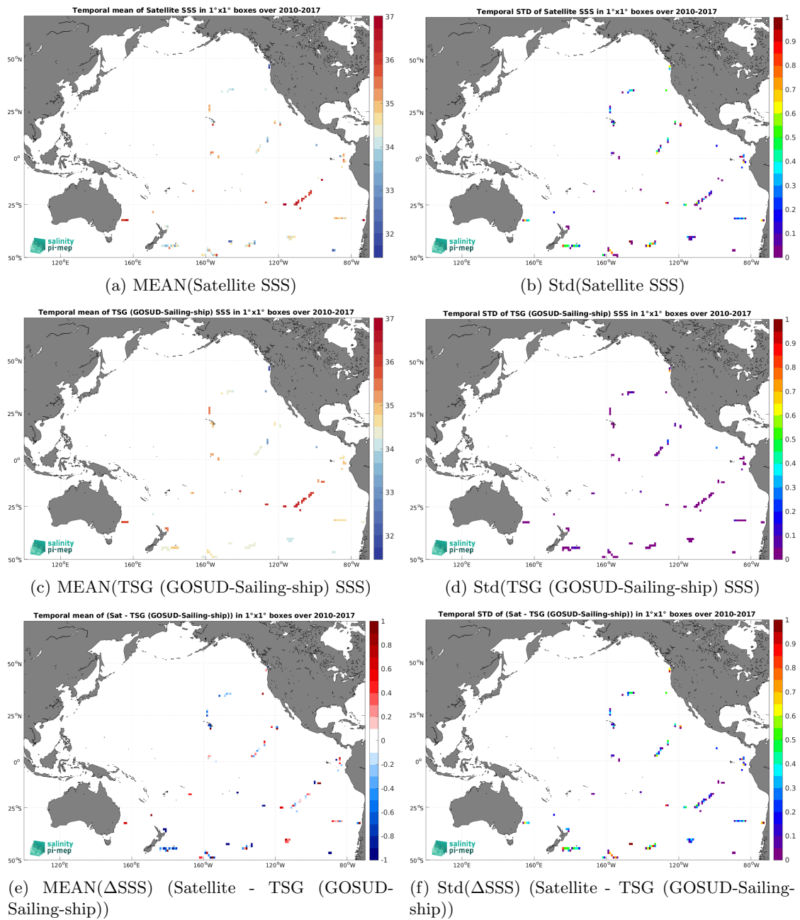
Figure 6: Temporal mean (left) and Std (right) of SSS from SMOS SSS L2Q v331 - 0.25 Deg (CATDS-CPDC) (top), TSG (GOSUD-Sailing-ship) (middle), and of \Delta SSS (Satellite - TSG (GOSUD-Sailing-ship)). Only match-up pairs are used to generate these maps.
