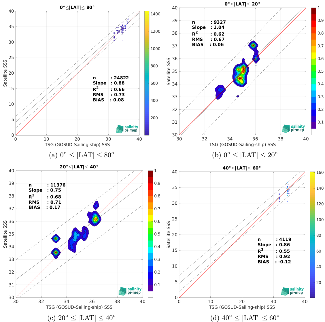
Figure 9: Contour maps of the concentration of SMOS SSS L2Q v331 - 0.25 Deg (CATDS-CPDC) SSS (y-axis) versus TSG (GOSUD-Sailing-ship) SSS (x-axis) at match-up pairs for different latitude bands. For each plot, the red line shows x=y . The black thin and dashed lines indicate a linear fit through the data cloud and the \pm 95\% confidence levels, respectively. The number match-up pairs n , the slope and R^2 coefficient of the linear fit, the root mean square (RMS) and the mean bias between satellite and in situ data are indicated for each latitude band in each plots.
