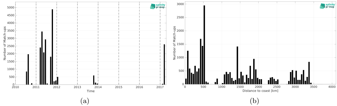
Figure 1: Number of match-ups between TSG (GOSUD-Sailing-ship) and SMOS SSS L2Q v331 - 0.25 Deg (CATDS-CPDC) SSS as a function of time (a) and as function of the distance to coast (b) over the Pacific Ocean Pi-MEP region and for the full satellite product period.
