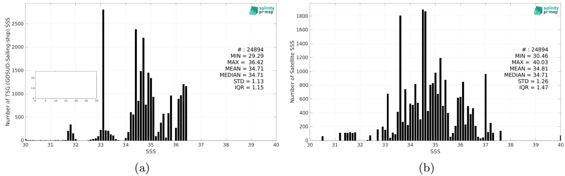
Figure 2: Histograms of SSS from TSG (GOSUD-Sailing-ship) (a) and SMOS SSS L2Q v331 - 0.25 Deg (CATDS-CPDC) (b) considering all match-up pairs per bins of 0.1 over the Pacific Ocean Pi-MEP region and for the full satellite product period.
