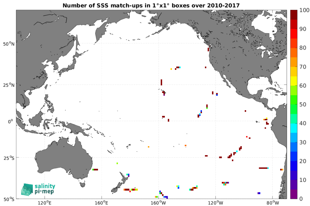
Figure 4: Number of SSS match-ups between TSG (GOSUD-Sailing-ship) SSS and the SMOS SSS L2Q v331 - 0.25 Deg (CATDS-CPDC) SSS product for the Pacific Ocean Pi-MEP region over 1^\circ \times 1^\circ boxes and for the full satellite product period.
