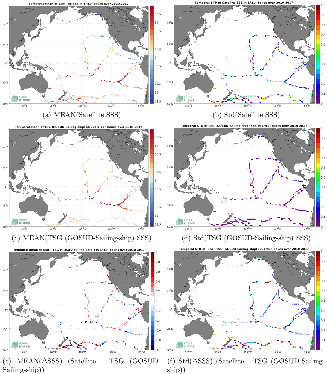
Figure 6: Temporal mean (left) and Std (right) of SSS from SMOS SSS L2Q v331 - 0.25 Deg (CATDS-CPDC) (top), TSG (GOSUD-Sailing-ship) (middle), and of ΔSSS (Satellite - TSG (GOSUD-Sailing-ship)). Only match-up pairs are used to generate these maps.
