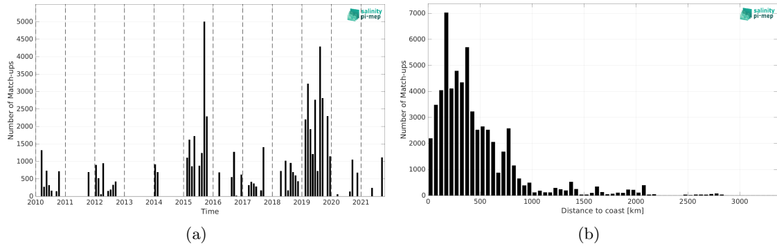
Figure 1: Number of match-ups between TSG (GOSUD-Research-vessel) and SMOS SSS L2Q v331 - 0.25 Deg (CATDS-CPDC) SSS as a function of time (a) and as function of the distance to coast (b) over the Pacific Ocean Pi-MEP region and for the full satellite product period.
