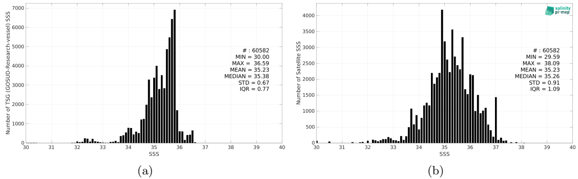
Figure 2: Histograms of SSS from TSG (GOSUD-Research-vessel) (a) and SMOS SSS L2Q v331 - 0.25 Deg (CATDS-CPDC) (b) considering all match-up pairs per bins of 0.1 over the Pacific Ocean Pi-MEP region and for the full satellite product period.
