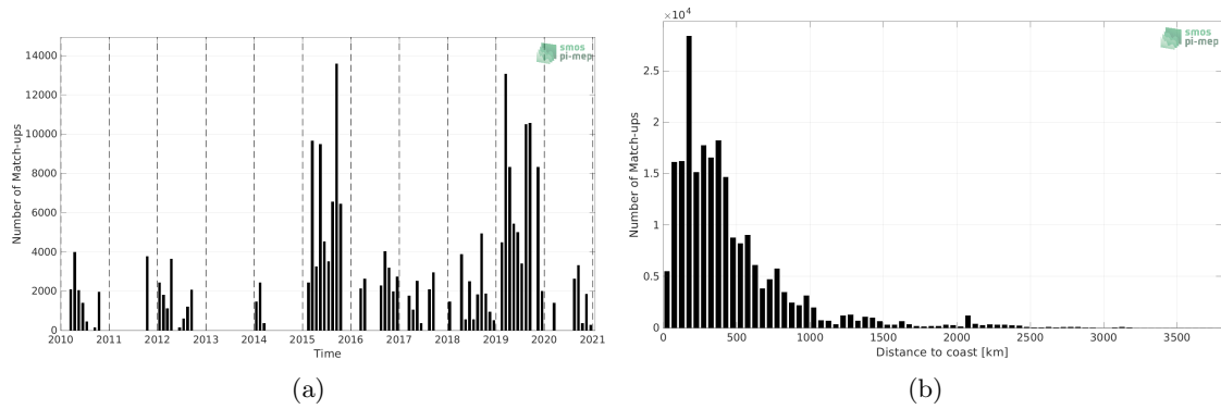
Figure 1: Number of match-ups between TSG (GOSUD-Research-vessel) and SMOS SSS L2Q v331 - 0.25 Deg (CATDS-CPDC) SSS as a function of time (a) and as function of the distance to coast (b) over the Pacific Ocean Pi-MEP region and for the full satellite product period.
