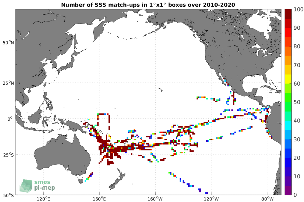
Figure 4: Number of SSS match-ups between TSG (GOSUD-Research-vessel) SSS and the SMOS SSS L2Q v331 - 0.25 Deg (CATDS-CPDC) SSS product for the Pacific Ocean Pi-MEP region over 1^\circ \times 1^\circ boxes and for the full satellite product period.
