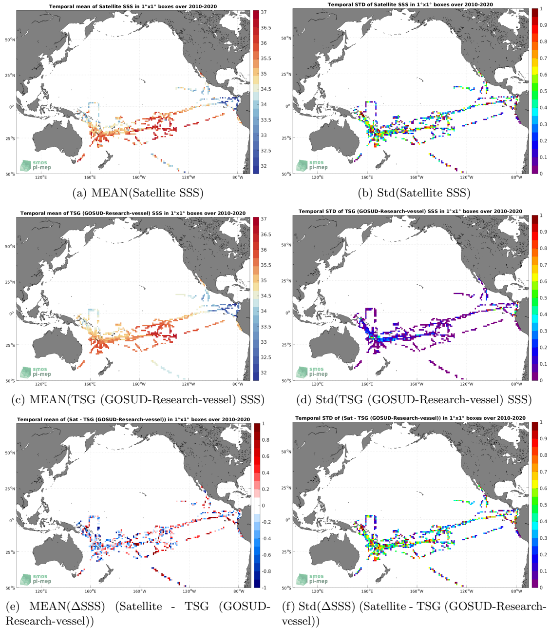
Figure 6: Temporal mean (left) and Std (right) of SSS from SMOS SSS L2Q v331 - 0.25 Deg (CATDS-CPDC) (top), TSG (GOSUD-Research-vessel) (middle), and of \Delta SSS (Satellite - TSG (GOSUD-Research-vessel)). Only match-up pairs are used to generate these maps.
