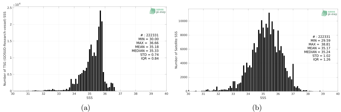
Figure 2: Histograms of SSS from TSG (GOSUD-Research-vessel) (a) and SMOS SSS L2Q v331 - 0.25 Deg (CATDS-CPDC) (b) considering all match-up pairs per bins of 0.1 over the Pacific Ocean Pi-MEP region and for the full satellite product period.
