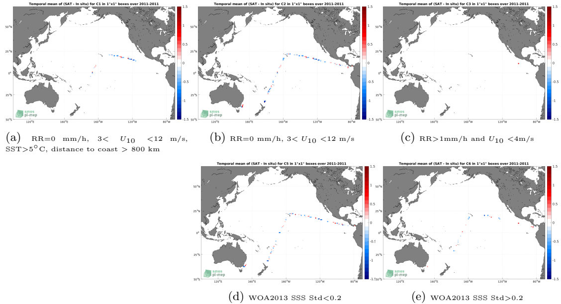
Figure 12: Temporal mean gridded over spatial boxes of size 1^{\circ}\times 1^{\circ} of \Delta\text{SSS} (SMOS SSS L2Q v331 - 0.25 Deg (CATDS-CPDC) - TSG (CSIC-UTM)) for 5 different subdatasets corresponding to:RR=0 mm/h, 3 < U_{10} < 12 m/s, SST >5^{\circ}\text{C} , distance to coast > 800 km (a), RR=0 mm/h, 3 < U_{10} < 12 m/s (b), RR >1 mm/h and U_{10} < 4 m/s (c), WOA2013 SSS Std <0.2 (d), WOA2013 SSS Std >0.2 (e).
