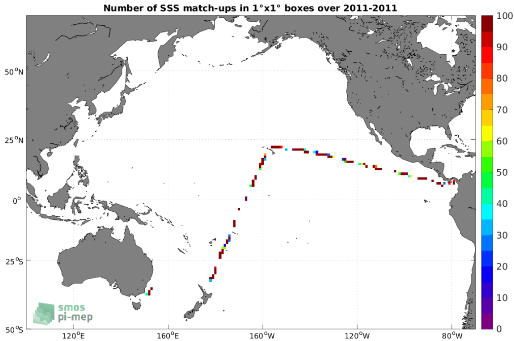
Figure 4: Number of SSS match-ups between TSG (CSIC-UTM) SSS and the SMOS SSS L2Q v331 - 0.25 Deg (CATDS-CPDC) SSS product for the Pacific Ocean Pi-MEP region over 1^\circ \times 1^\circ boxes and for the full satellite product period.
