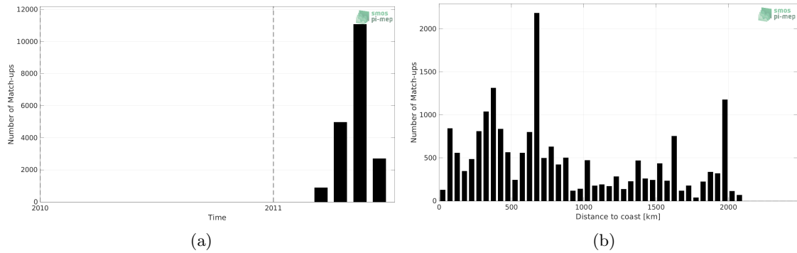
Figure 1: Number of match-ups between TSG (CSIC-UTM) and SMOS SSS L2Q v331 - 0.25 Deg (CATDS-CPDC) SSS as a function of time (a) and as function of the distance to coast (b) over the Pacific Ocean Pi-MEP region and for the full satellite product period.
