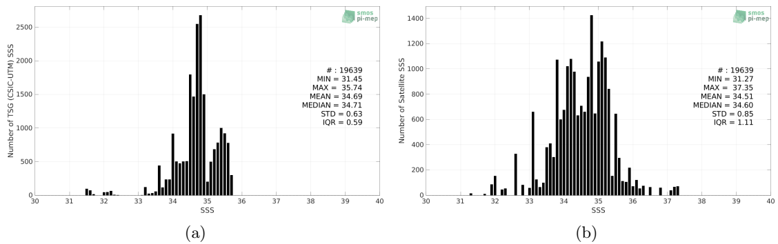
Figure 2: Histograms of SSS from TSG (CSIC-UTM) (a) and SMOS SSS L2Q v331 - 0.25 Deg (CATDS-CPDC) (b) considering all match-up pairs per bins of 0.1 over the Pacific Ocean Pi-MEP region and for the full satellite product period.
