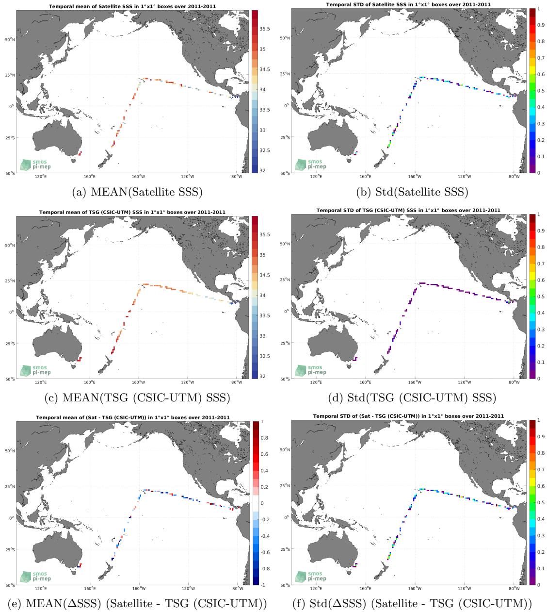
Figure 6: Temporal mean (left) and Std (right) of SSS from SMOS SSS L2Q v331 - 0.25 Deg (CATDS-CPDC) (top), TSG (CSIC-UTM) (middle), and of \Delta SSS (Satellite - TSG (CSIC-UTM)). Only match-up pairs are used to generate these maps.
