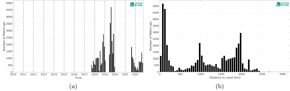
Figure 1: Number of match-ups between Saildrone and SMOS SSS L2Q v331 - 0.25 Deg (CATDS-CPDC) SSS as a function of time (a) and as function of the distance to coast (b) over the Pacific Ocean Pi-MEP region and for the full satellite product period.
