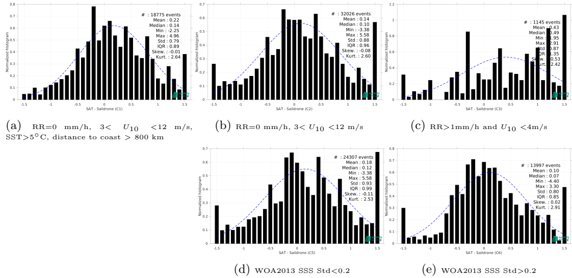
Figure 13: Normalized histogram of \Delta SSS (SMOS SSS L2Q v331 - 0.25 Deg (CATDS-CPDC) - Saildrone) for 5 different subdatasets corresponding to: RR=0 mm/h, 3 < U_{10} < 12 m/s, SST > 5°C, distance to coast > 800 km (a), RR=0 mm/h, 3 < U_{10} < 12 m/s (b), RR > 1mm/h and U_{10} < 4 m/s (c), WOA2013 SSS Std < 0.2 (d), WOA2013 SSS Std > 0.2 (e).
