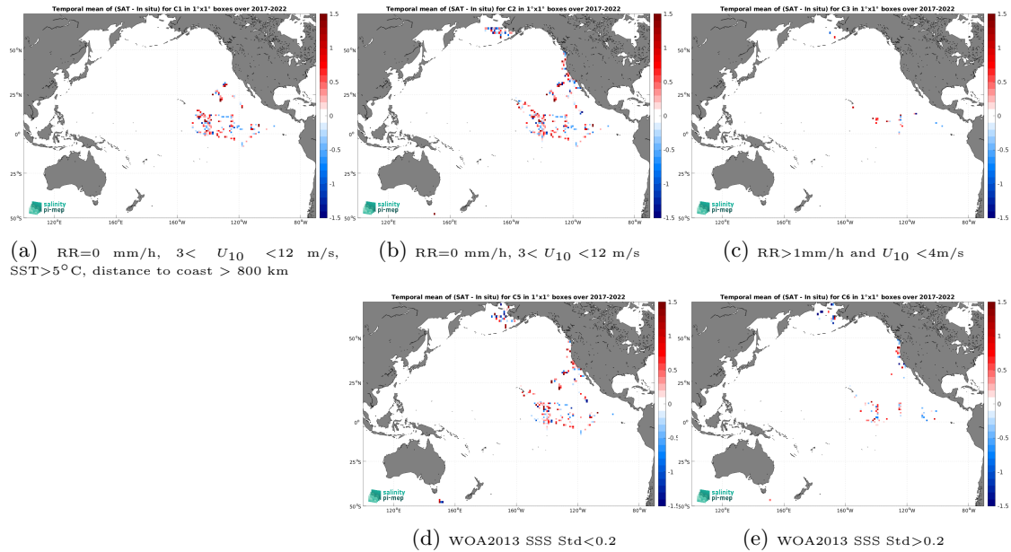
Figure 12: Temporal mean gridded over spatial boxes of size 1^\circ \times 1^\circ of \Delta SSS (SMOS SSS L2Q v331 - 0.25 Deg (CATDS-CPDC) - Saildrone) for 5 different subdatasets corresponding to:RR=0 mm/h, 3 < U_{10} < 12 m/s, SST >5^\circ C, distance to coast > 800 km (a), RR=0 mm/h, 3 < U_{10} < 12 m/s (b), RR >1 mm/h and U_{10} < 4 m/s (c), WOA2013 SSS Std <0.2 (d), WOA2013 SSS Std >0.2 (e).
