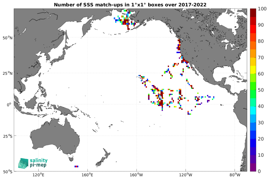
Figure 4: Number of SSS match-ups between Saildrone SSS and the SMOS SSS L2Q v331 - 0.25 Deg (CATDS-CPDC) SSS product for the Pacific Ocean Pi-MEP region over 1^\circ \times 1^\circ boxes and for the full satellite product period.
