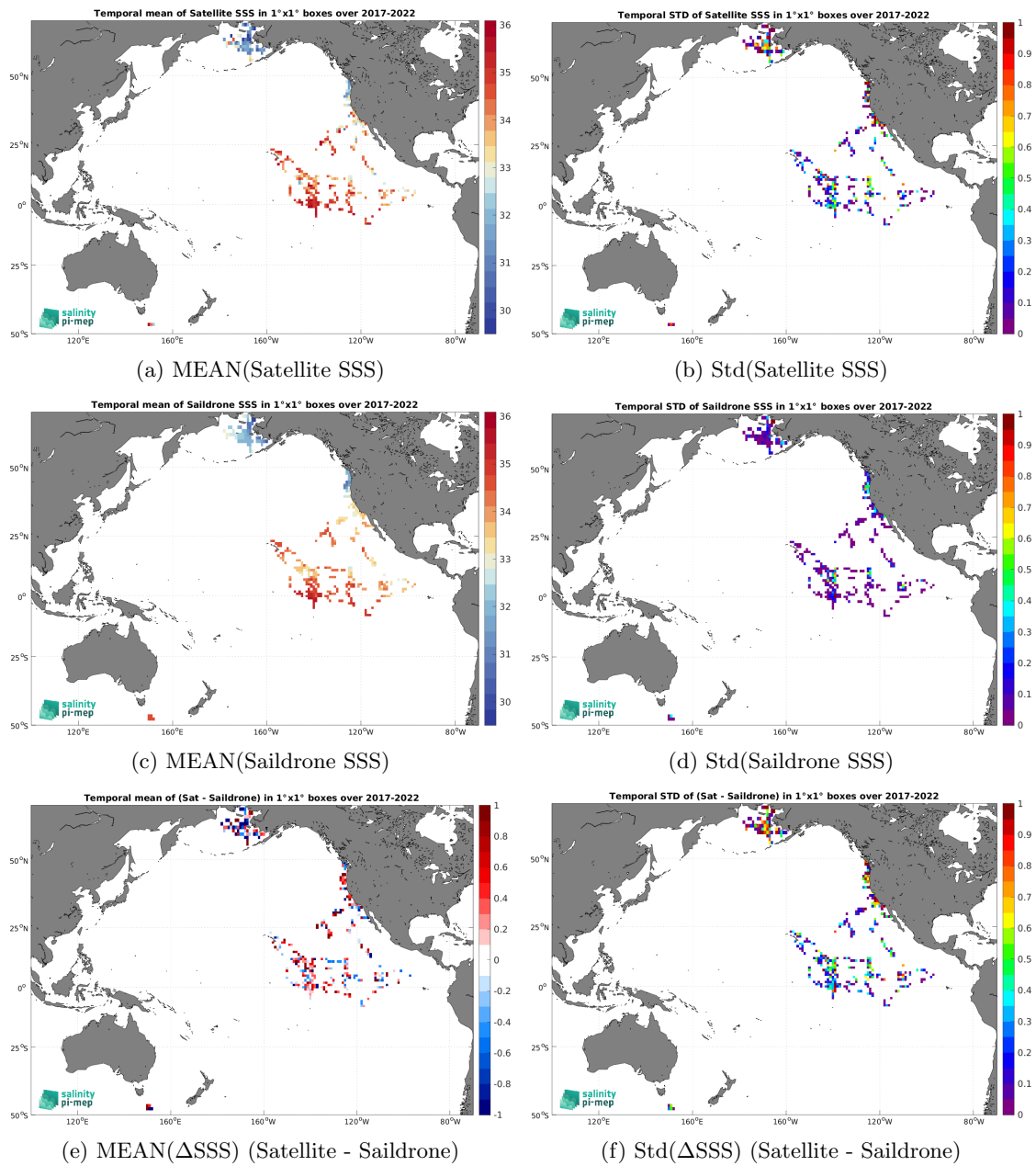
Figure 6: Temporal mean (left) and Std (right) of SSS from SMOS SSS L2Q v331 - 0.25 Deg (CATDS-CPDC) (top), Saildrone (middle), and of \Delta SSS (Satellite - Saildrone). Only match-up pairs are used to generate these maps.
