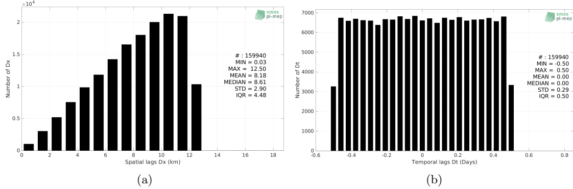
Figure 5: Histograms of the spatial (a) and temporal (b) lags between the location/time of the Saildrone measurement and the date of the corresponding SMOS SSS L2Q v331 - 0.25 Deg (CATDS-CPDC) SSS pixel.
