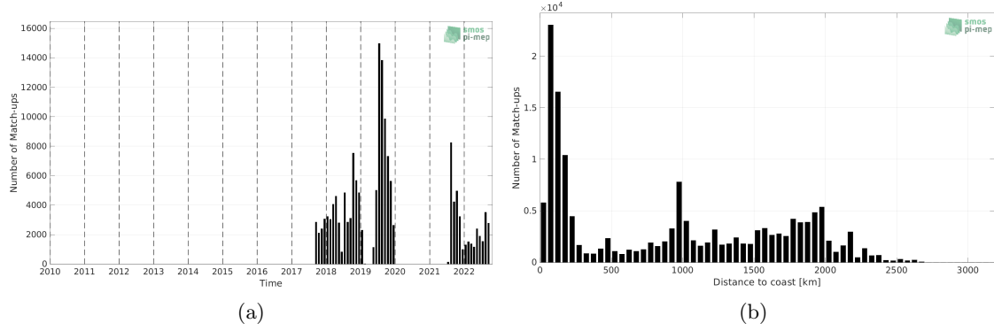
Figure 1: Number of match-ups between Saildrone and SMOS SSS L2Q v331 - 0.25 Deg (CATDS-CPDC) SSS as a function of time (a) and as function of the distance to coast (b) over the Pacific Ocean Pi-MEP region and for the full satellite product period.
