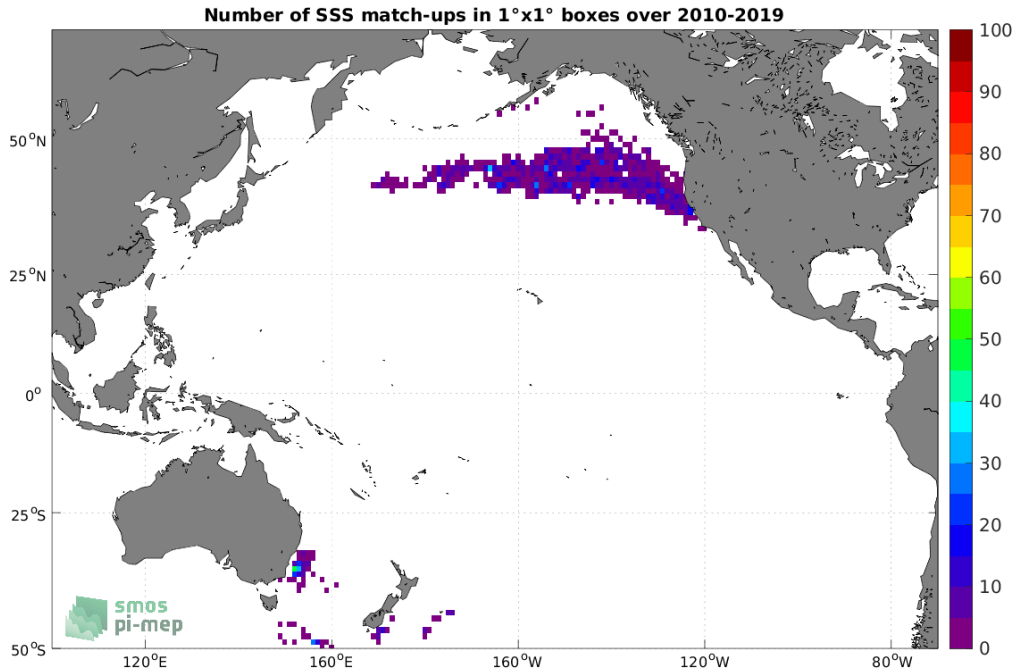
Figure 4: Number of SSS match-ups between Marine mammals SSS and the SMOS SSS L2Q v331 - 0.25 Deg (CATDS-CPDC) SSS product for the Pacific Ocean Pi-MEP region over 1^\circ \times 1^\circ boxes and for the full satellite product period.
