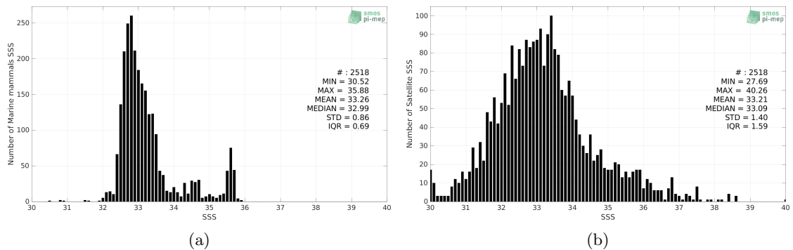
Figure 2: Histograms of SSS from Marine mammals (a) and SMOS SSS L2Q v331 - 0.25 Deg (CATDS-CPDC) (b) considering all match-up pairs per bins of 0.1 over the Pacific Ocean Pi-MEP region and for the full satellite product period.
