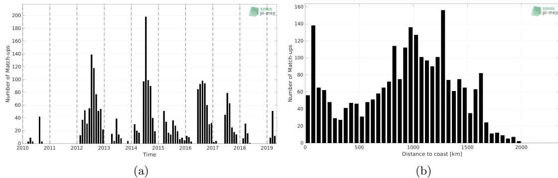
Figure 1: Number of match-ups between Marine mammals and SMOS SSS L2Q v331 - 0.25 Deg (CATDS-CPDC) SSS as a function of time (a) and as function of the distance to coast (b) over the Pacific Ocean Pi-MEP region and for the full satellite product period.
