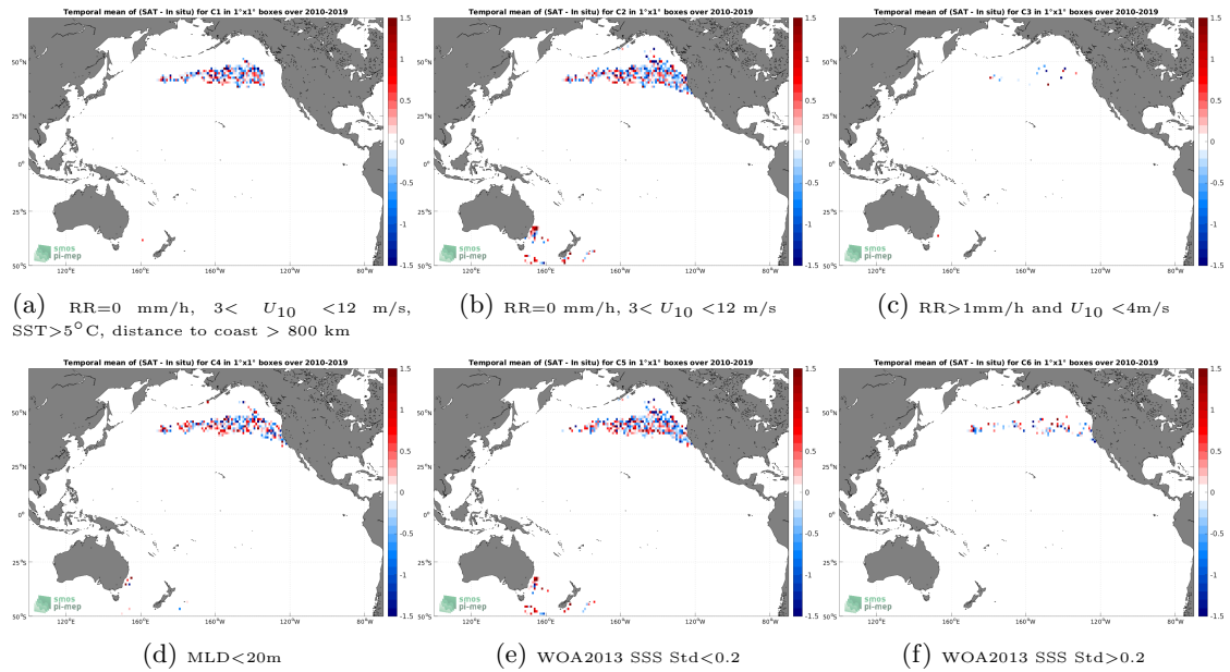
Figure 12: Temporal mean gridded over spatial boxes of size 1^\circ \times 1^\circ of \Delta SSS (SMOS SSS L2Q v331 - 0.25 Deg (CATDS-CPDC) - Marine mammals) for 6 different subdatasets corresponding to:RR=0 mm/h, 3 < U_{10} < 12 m/s, SST > 5^\circ\text{C} , distance to coast > 800 km (a), RR=0 mm/h, 3 < U_{10} < 12 m/s (b), RR > 1 mm/h and U_{10} < 4 m/s (c),MLD < 20 m (d),WOA2013 SSS Std < 0.2 (e),WOA2013 SSS Std > 0.2 (f).
