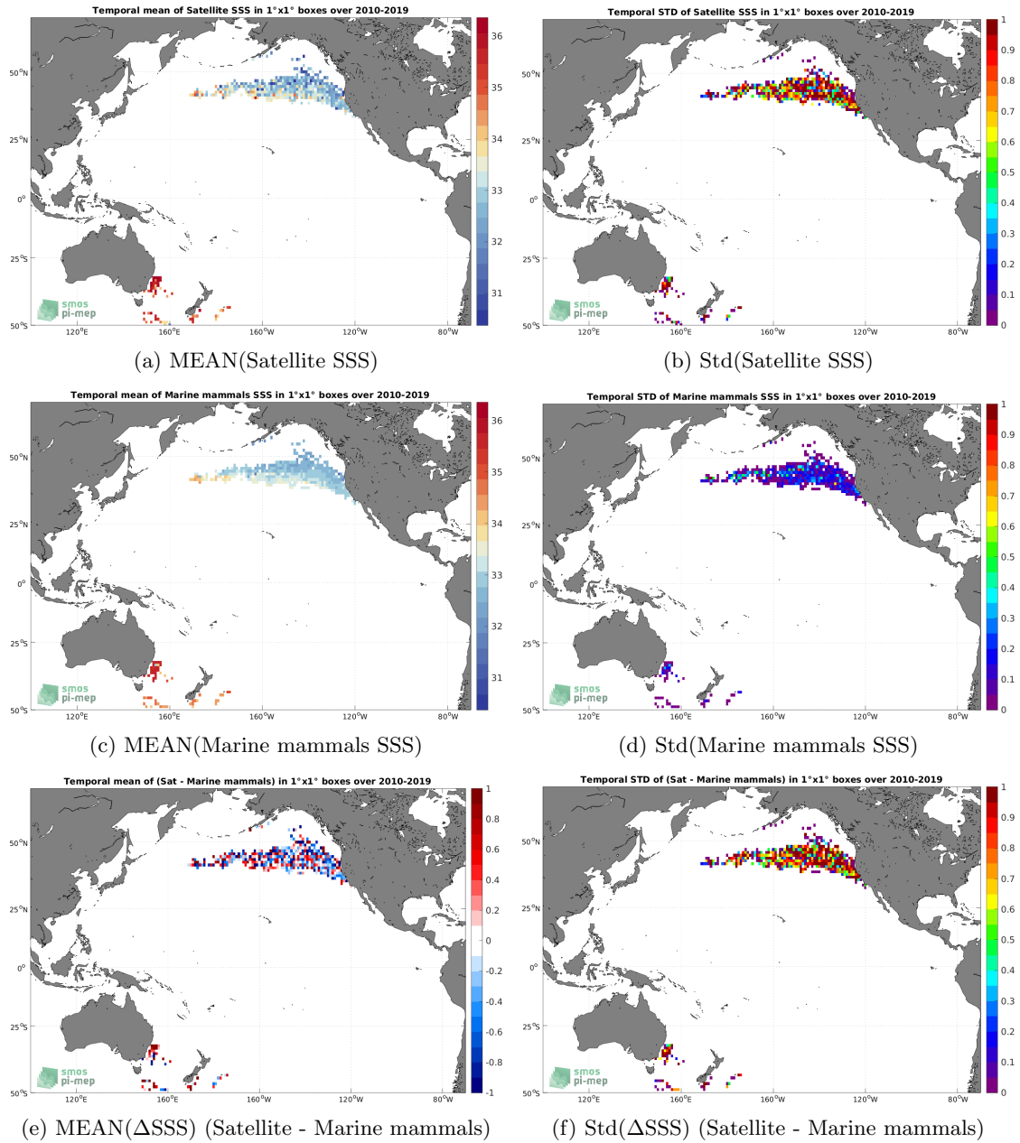
Figure 6: Temporal mean (left) and Std (right) of SSS from SMOS SSS L2Q v331 - 0.25 Deg (CATDS-CPDC) (top), Marine mammals (middle), and of \Delta SSS (Satellite - Marine mammals). Only match-up pairs are used to generate these maps.
