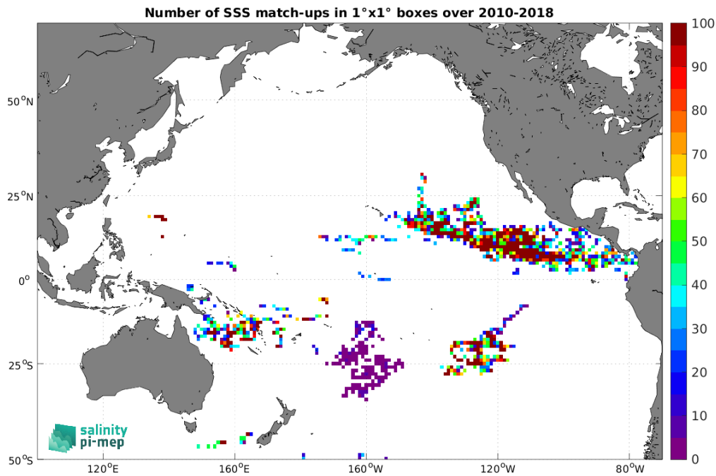
Figure 3: Number of SSS match-ups between Surface drifters SSS and the SMOS SSS L2Q v331 - 0.25 Deg (CATDS-CPDC) SSS product for the Pacific Ocean Pi-MEP region over 1^\circ \times 1^\circ boxes and for the full satellite product period.
