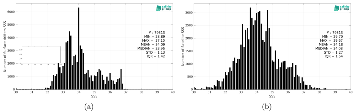
Figure 2: Histograms of SSS from Surface drifters (a) and SMOS SSS L2Q v331 - 0.25 Deg (CATDS-CPDC) (b) considering all match-up pairs per bins of 0.1 over the Pacific Ocean Pi-MEP region and for the full satellite product period.
