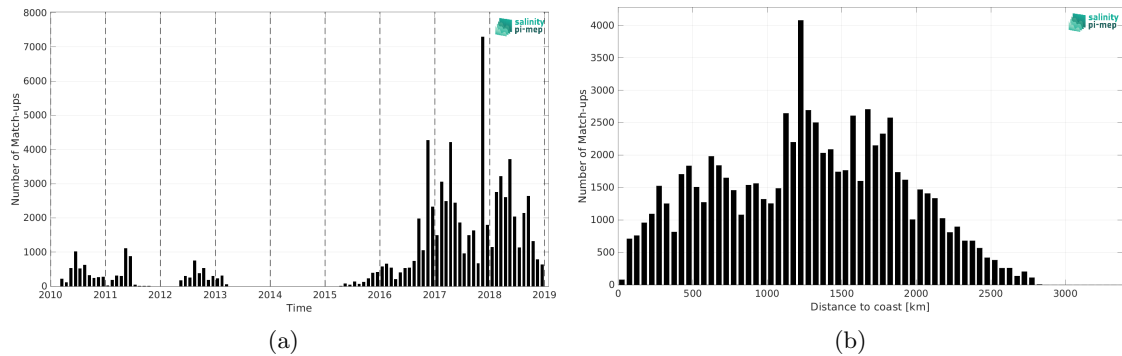
Figure 1: Number of match-ups between Surface drifters and SMOS SSS L2Q v331 - 0.25 Deg (CATDS-CPDC) SSS as a function of time (a) and as function of the distance to coast (b) over the Pacific Ocean Pi-MEP region and for the full satellite product period.
