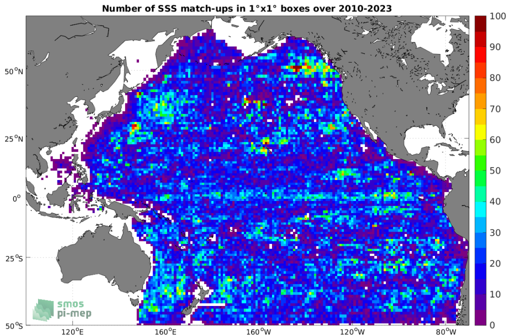
Figure 4: Number of SSS match-ups between Argo SSS and the SMOS SSS L2Q v331 - 0.25 Deg (CATDS-CPDC) SSS product for the Pacific Ocean Pi-MEP region over 1^\circ \times 1^\circ boxes and for the full satellite product period.
