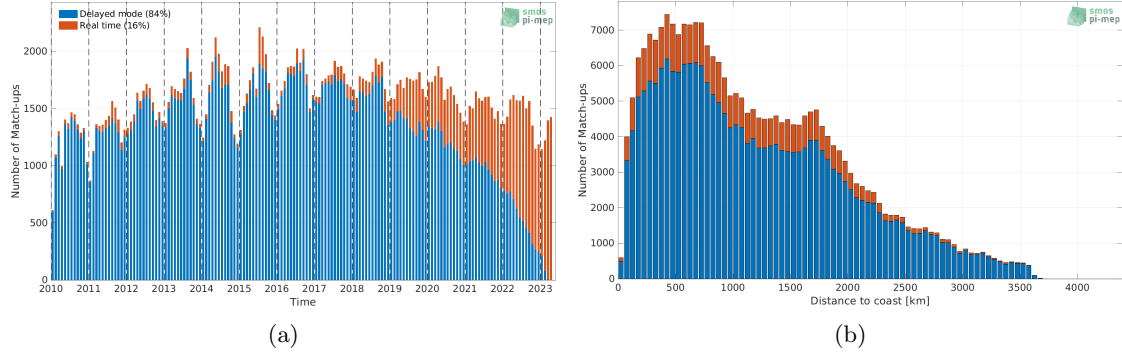
Figure 1: Number of match-ups between Argo and SMOS SSS L2Q v331 - 0.25 Deg (CATDS-CPDC) SSS as a function of time (a) and as function of the distance to coast (b) over the Pacific Ocean Pi-MEP region and for the full satellite product period.
