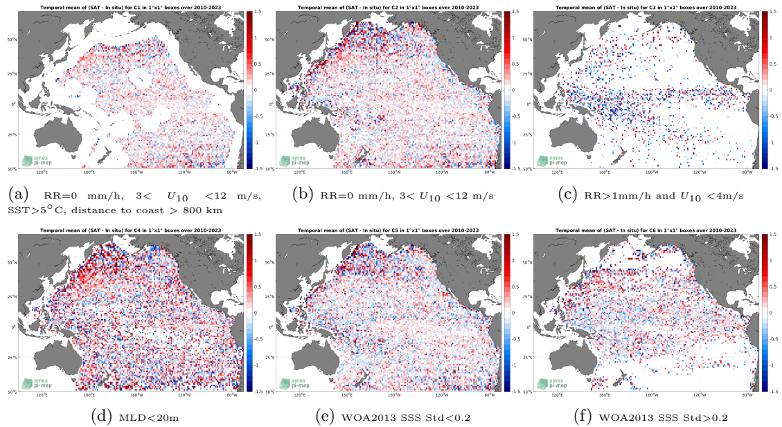
Figure 12: Temporal mean gridded over spatial boxes of size 1^\circ \times 1^\circ of \Delta SSS (SMOS SSS L2Q v331 - 0.25 Deg (CATDS-CPDC) - Argo) for 6 different subdatasets corresponding to:RR=0 mm/h, 3 < U_{10} < 12 m/s, SST > 5^\circ\text{C} , distance to coast > 800 km (a), RR=0 mm/h, 3 < U_{10} < 12 m/s (b), RR > 1 mm/h and U_{10} < 4 m/s (c),MLD < 20 m (d),WOA2013 SSS Std < 0.2 (e),WOA2013 SSS Std > 0.2 (f).
