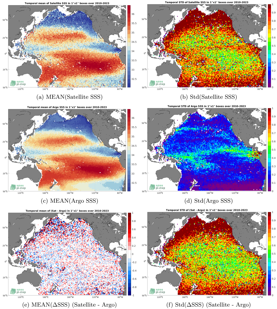
Figure 6: Temporal mean (left) and Std (right) of SSS from SMOS SSS L2Q v331 - 0.25 Deg (CATDS-CPDC) (top), Argo (middle), and of \Delta SSS (Satellite - Argo). Only match-up pairs are used to generate these maps.
