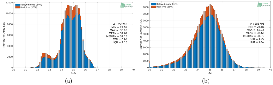
Figure 2: Histograms of SSS from Argo (a) and SMOS SSS L2Q v331 - 0.25 Deg (CATDS-CPDC) (b) considering all match-up pairs per bins of 0.1 over the Pacific Ocean Pi-MEP region and for the full satellite product period.
