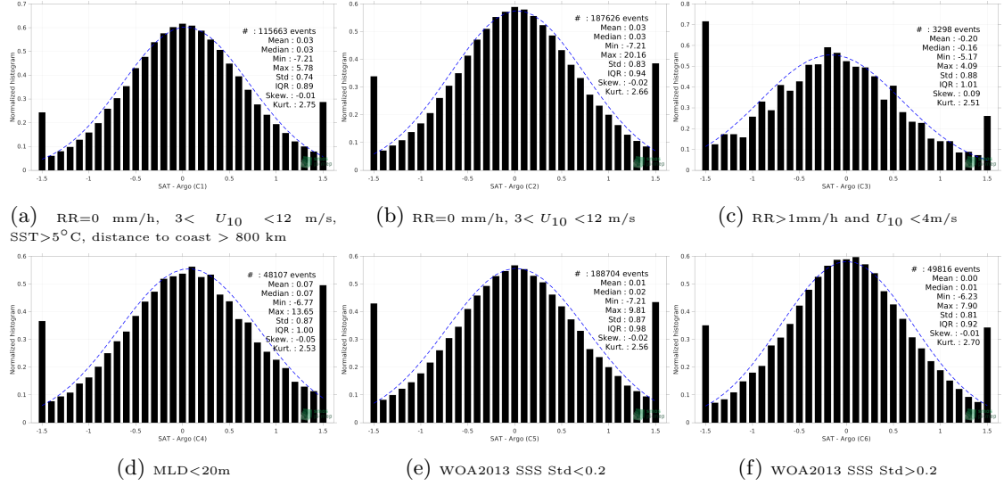
Figure 13: Normalized histogram of \Delta SSS (SMOS SSS L2Q v331 - 0.25 Deg (CATDS-CPDC) - Argo) for 6 different subdatasets corresponding to: RR=0 mm/h, 3 < U_{10} < 12 m/s, SST>5°C, distance to coast > 800 km (a), RR=0 mm/h, 3 < U_{10} < 12 m/s (b), RR>1mm/h and U_{10} < 4 m/s (c), MLD<20m (d), WOA2013 SSS Std<0.2 (e), WOA2013 SSS Std>0.2 (f).
