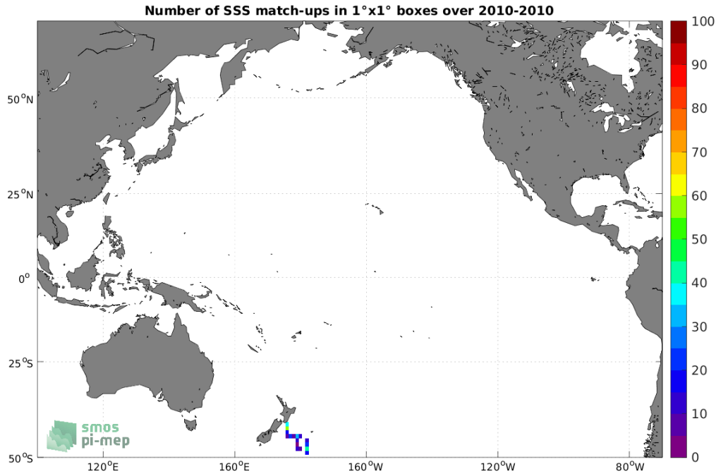
Figure 4: Number of SSS match-ups between TSG (Polarstern) SSS and the SMOS SSS L2Q v330 - 0.25 Deg (CATDS-CPDC) SSS product for the Pacific Ocean Pi-MEP region over 1^\circ \times 1^\circ boxes and for the full satellite product period.
