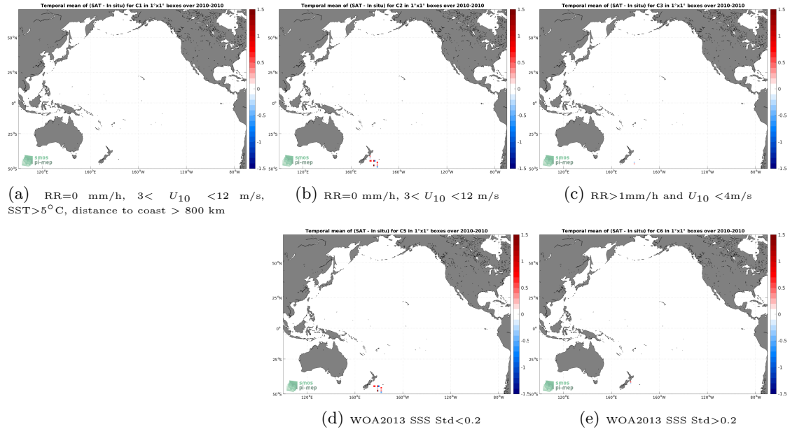
Figure 12: Temporal mean gridded over spatial boxes of size 1^{\circ}\times 1^{\circ} of \Delta\text{SSS} (SMOS SSS L2Q v330 - 0.25 Deg (CATDS-CPDC) - TSG (Polarstern)) for 5 different subdatasets corresponding to:RR=0 mm/h, 3 < U_{10} < 12 m/s, SST >5^{\circ}\text{C} , distance to coast > 800 km (a), RR=0 mm/h, 3 < U_{10} < 12 m/s (b), RR >1 mm/h and U_{10} < 4 m/s (c), WOA2013 SSS Std <0.2 (d), WOA2013 SSS Std >0.2 (e).
