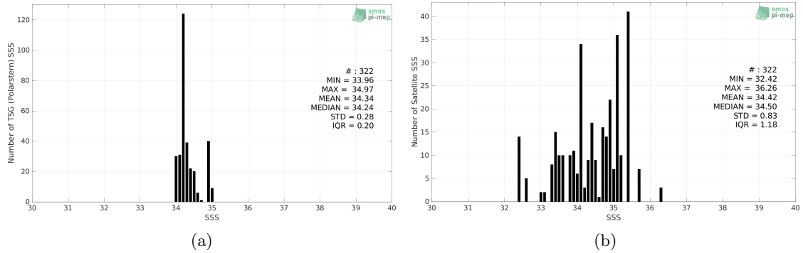
Figure 2: Histograms of SSS from TSG (Polarstern) (a) and SMOS SSS L2Q v330 - 0.25 Deg (CATDS-CPDC) (b) considering all match-up pairs per bins of 0.1 over the Pacific Ocean Pi-MEP region and for the full satellite product period.
