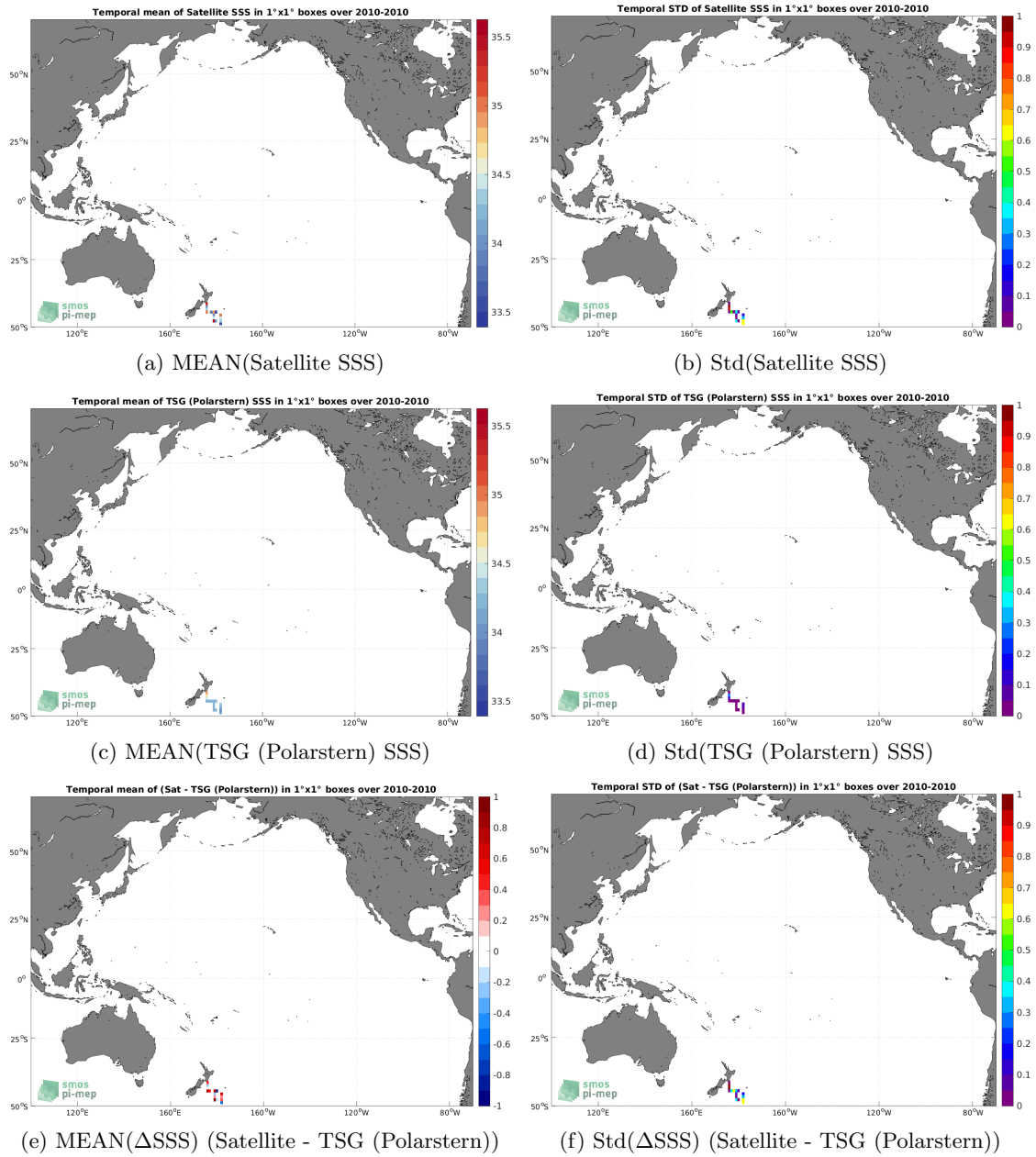
Figure 6: Temporal mean (left) and Std (right) of SSS from SMOS SSS L2Q v330 - 0.25 Deg (CATDS-CPDC) (top), TSG (Polarstern) (middle), and of \Delta SSS (Satellite - TSG (Polarstern)). Only match-up pairs are used to generate these maps.
