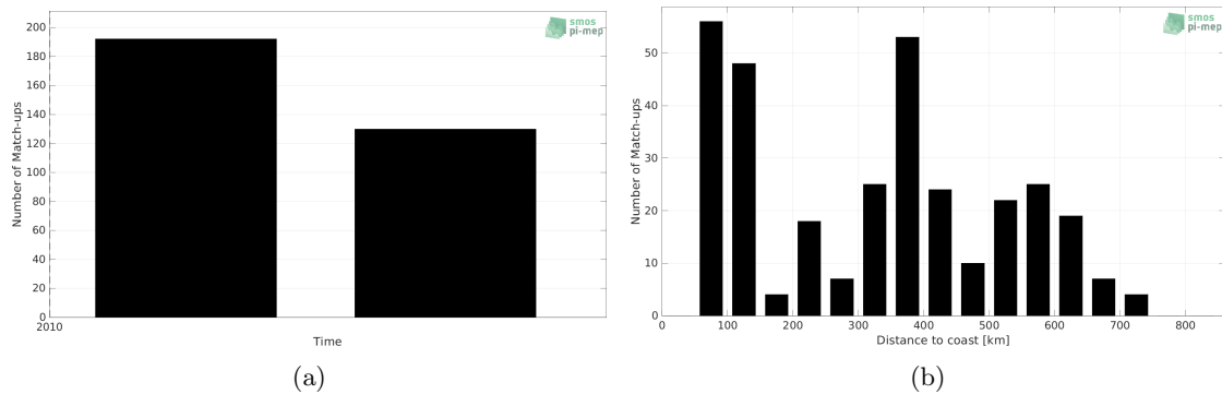
Figure 1: Number of match-ups between TSG (Polarstern) and SMOS SSS L2Q v330 - 0.25 Deg (CATDS-CPDC) SSS as a function of time (a) and as function of the distance to coast (b) over the Pacific Ocean Pi-MEP region and for the full satellite product period.
