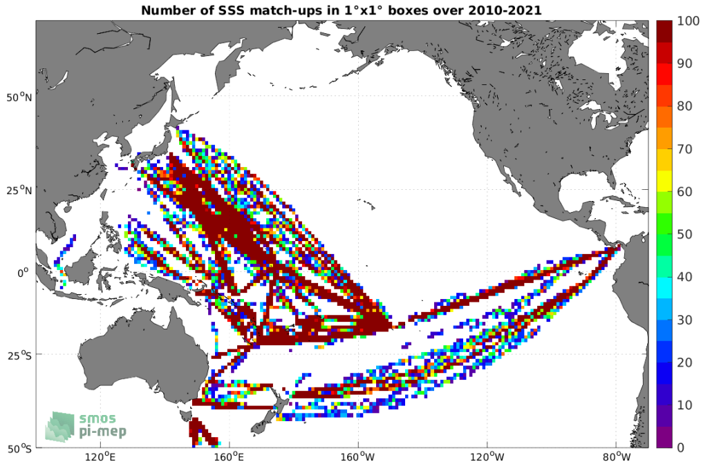
Figure 4: Number of SSS match-ups between TSG (LEGOS-DM) SSS and the SMOS SSS L2Q v330 - 0.25 Deg (CATDS-CPDC) SSS product for the Pacific Ocean Pi-MEP region over 1^\circ \times 1^\circ boxes and for the full satellite product period.
