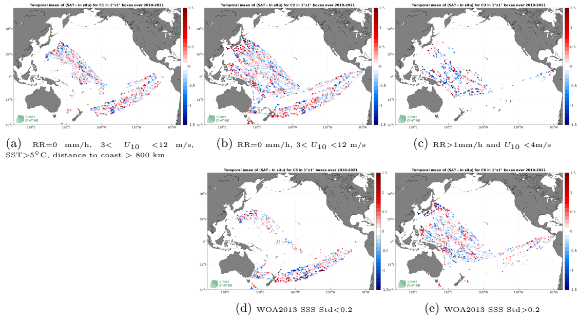
Figure 12: Temporal mean gridded over spatial boxes of size 1^\circ \times 1^\circ of \Delta SSS (SMOS SSS L2Q v330 - 0.25 Deg (CATDS-CPDC) - TSG (LEGOS-DM)) for 5 different subdatasets corresponding to:RR=0 mm/h, 3 < U_{10} < 12 m/s, SST >5^\circ C, distance to coast > 800 km (a), RR=0 mm/h, 3 < U_{10} < 12 m/s (b), RR >1 mm/h and U_{10} < 4 m/s (c), WOA2013 SSS Std <0.2 (d), WOA2013 SSS Std >0.2 (e).
