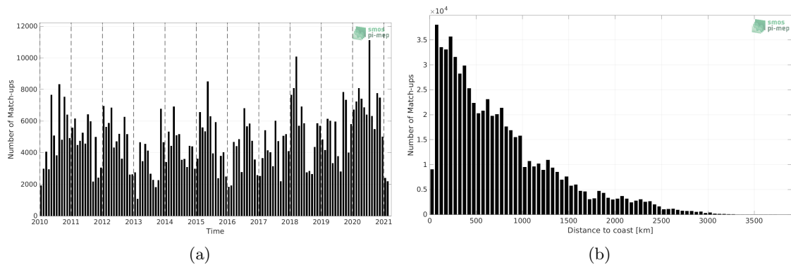
Figure 1: Number of match-ups between TSG (LEGOS-DM) and SMOS SSS L2Q v330 - 0.25 Deg (CATDS-CPDC) SSS as a function of time (a) and as function of the distance to coast (b) over the Pacific Ocean Pi-MEP region and for the full satellite product period.
