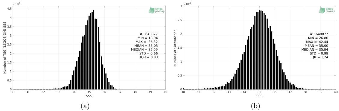
Figure 2: Histograms of SSS from TSG (LEGOS-DM) (a) and SMOS SSS L2Q v330 - 0.25 Deg (CATDS-CPDC) (b) considering all match-up pairs per bins of 0.1 over the Pacific Ocean Pi-MEP region and for the full satellite product period.
