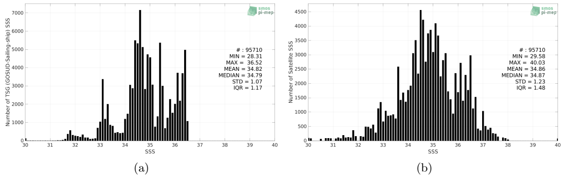
Figure 2: Histograms of SSS from TSG (GOSUD-Sailing-ship) (a) and SMOS SSS L2Q v330 - 0.25 Deg (CATDS-CPDC) (b) considering all match-up pairs per bins of 0.1 over the Pacific Ocean Pi-MEP region and for the full satellite product period.
