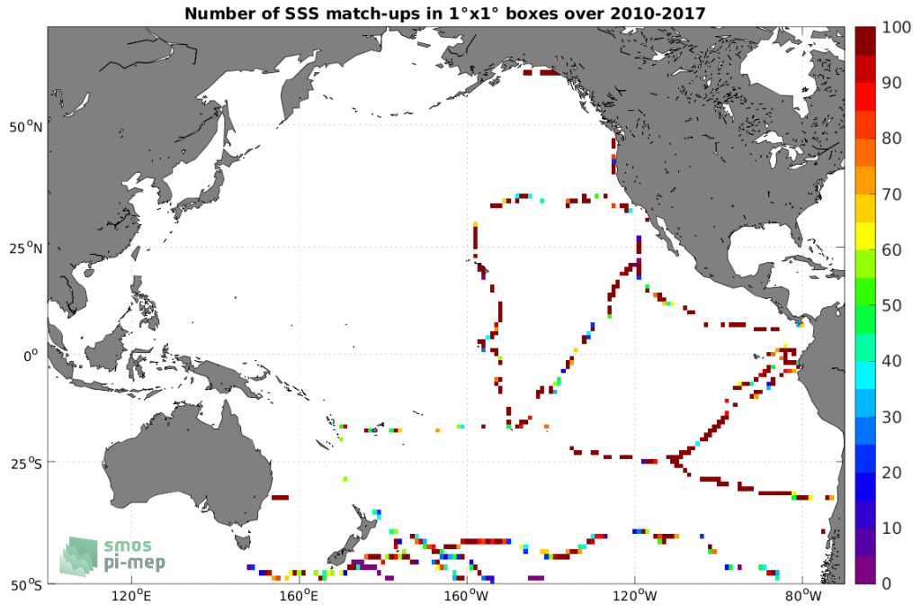
Figure 4: Number of SSS match-ups between TSG (GOSUD-Sailing-ship) SSS and the SMOS SSS L2Q v330 - 0.25 Deg (CATDS-CPDC) SSS product for the Pacific Ocean Pi-MEP region over 1^\circ \times 1^\circ boxes and for the full satellite product period.
