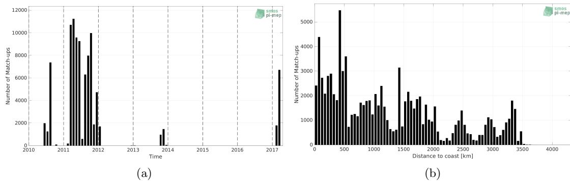
Figure 1: Number of match-ups between TSG (GOSUD-Sailing-ship) and SMOS SSS L2Q v330 - 0.25 Deg (CATDS-CPDC) SSS as a function of time (a) and as function of the distance to coast (b) over the Pacific Ocean Pi-MEP region and for the full satellite product period.
