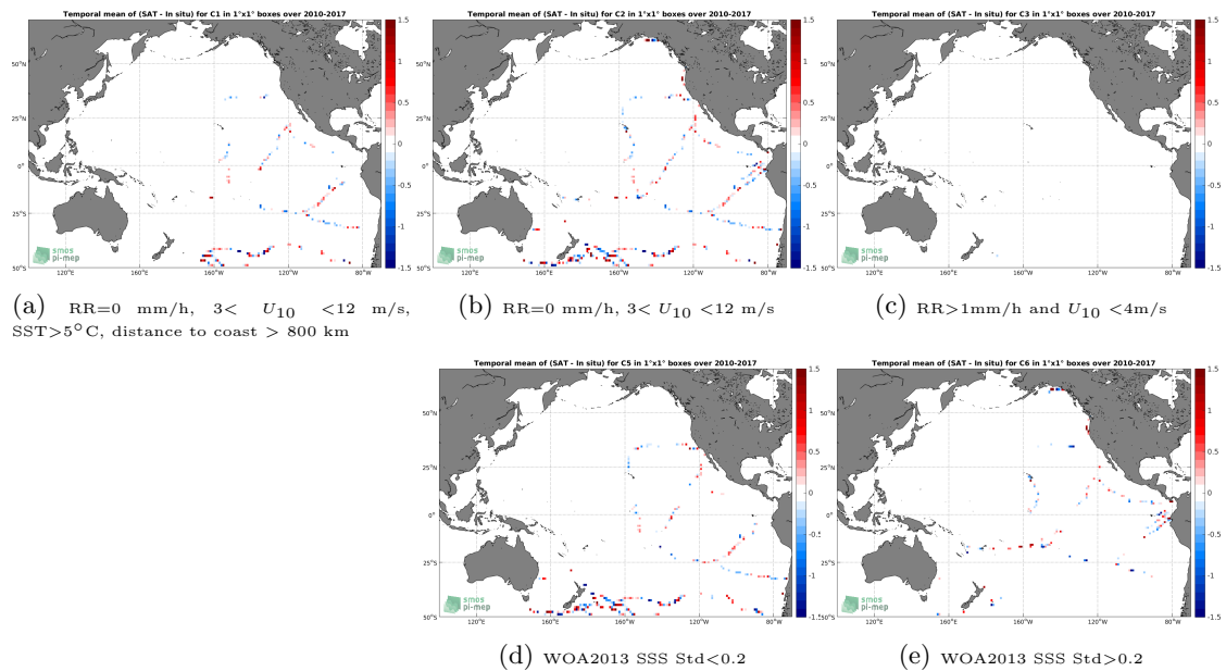
Figure 12: Temporal mean gridded over spatial boxes of size 1^\circ \times 1^\circ of \Delta\text{SSS} (SMOS SSS L2Q v330 - 0.25 Deg (CATDS-CPDC) - TSG (GOSUD-Sailing-ship)) for 5 different subdatasets corresponding to: RR=0 mm/h, 3 < U_{10} < 12 m/s, SST > 5°C, distance to coast > 800 km (a), RR=0 mm/h, 3 < U_{10} < 12 m/s (b), RR > 1mm/h and U_{10} < 4 m/s (c), WOA2013 SSS Std < 0.2 (d), WOA2013 SSS Std > 0.2 (e).
