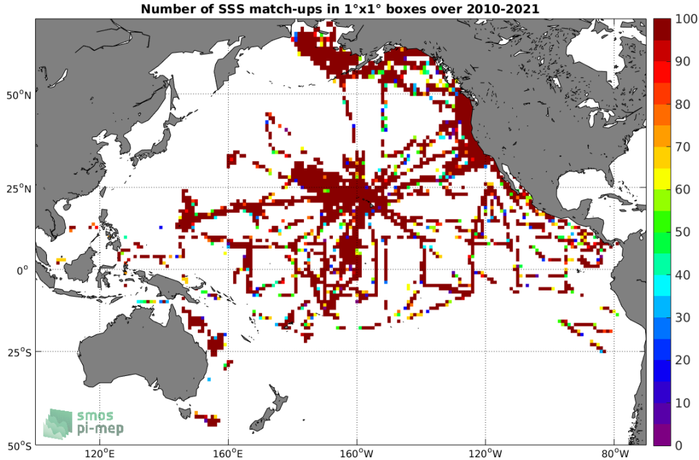
Figure 4: Number of SSS match-ups between TSG (SAMOS) SSS and the SMOS SSS L2Q v321 - 0.25 Deg (CATDS-CPDC) SSS product for the Pacific Ocean Pi-MEP region over 1°x1° boxes and for the full satellite product period.
