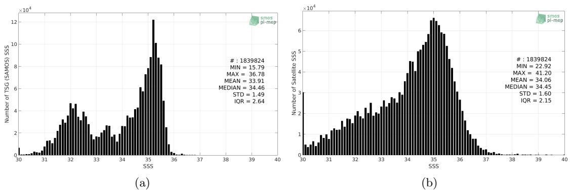
Figure 2: Histograms of SSS from TSG (SAMOS) (a) and SMOS SSS L2Q v321 - 0.25 Deg (CATDS-CPDC) (b) considering all match-up pairs per bins of 0.1 over the Pacific Ocean Pi-MEP region and for the full satellite product period.
