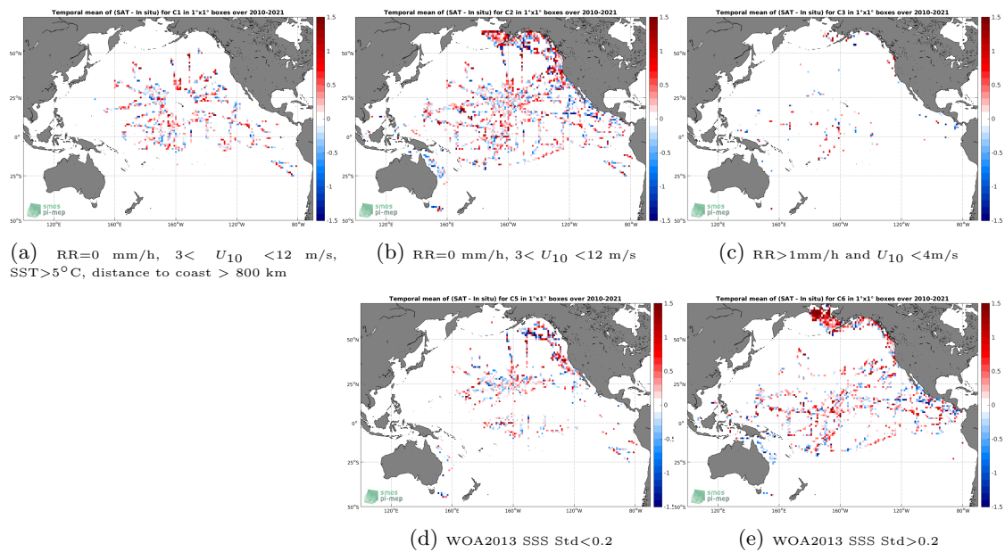
Figure 12: Temporal mean gridded over spatial boxes of size 1^\circ \times 1^\circ of \Delta\text{SSS} (SMOS SSS L2Q v321 - 0.25 Deg (CATDS-CPDC) - TSG (SAMOS)) for 5 different subdatasets corresponding to: RR=0 mm/h, 3 < U_{10} < 12 m/s, SST > 5°C, distance to coast > 800 km (a), RR=0 mm/h, 3 < U_{10} < 12 m/s (b), RR > 1mm/h and U_{10} < 4 m/s (c), WOA2013 SSS Std < 0.2 (d), WOA2013 SSS Std > 0.2 (e).
