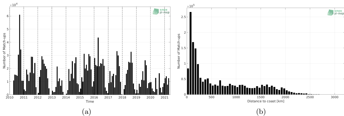
Figure 1: Number of match-ups between TSG (SAMOS) and SMOS SSS L2Q v321 - 0.25 Deg (CATDS-CPDC) SSS as a function of time (a) and as function of the distance to coast (b) over the Pacific Ocean Pi-MEP region and for the full satellite product period.
