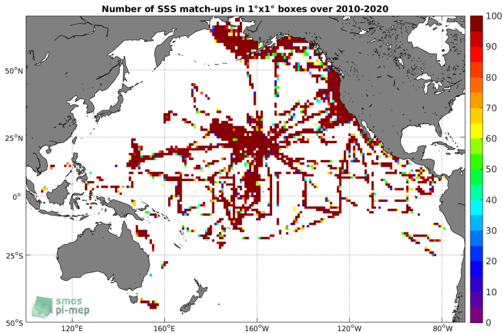
Figure 4: Number of SSS match-ups between TSG (SAMOS) SSS and the SMOS SSS L2Q v321 - 0.25 Deg (CATDS-CPDC) SSS product for the Pacific Ocean Pi-MEP region over 1^\circ \times 1^\circ boxes and for the full satellite product period.
