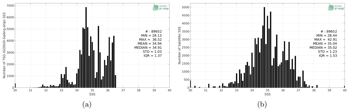
Figure 2: Histograms of SSS from TSG (GOSUD-Sailing-ship) (a) and SMOS SSS L2Q v321 - 0.25 Deg (CATDS-CPDC) (b) considering all match-up pairs per bins of 0.1 over the Pacific Ocean Pi-MEP region and for the full satellite product period.
