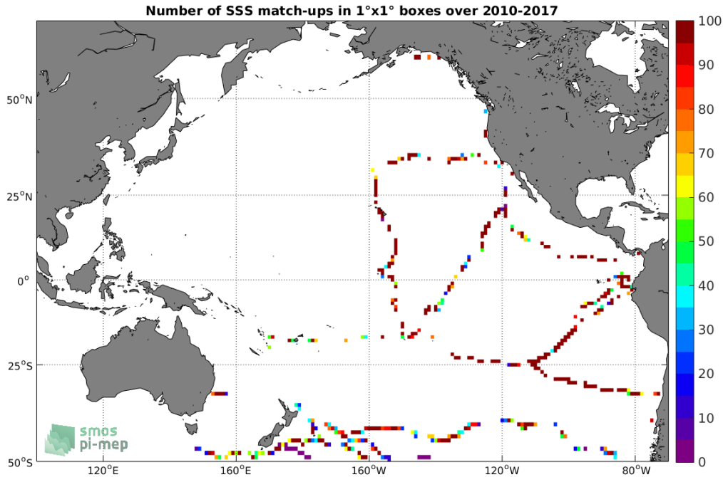
Figure 4: Number of SSS match-ups between TSG (GOSUD-Sailing-ship) SSS and the SMOS SSS L2Q v321 - 0.25 Deg (CATDS-CPDC) SSS product for the Pacific Ocean Pi-MEP region over 1^\circ \times 1^\circ boxes and for the full satellite product period.
