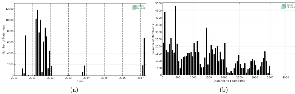
Figure 1: Number of match-ups between TSG (GOSUD-Sailing-ship) and SMOS SSS L2Q v321 - 0.25 Deg (CATDS-CPDC) SSS as a function of time (a) and as function of the distance to coast (b) over the Pacific Ocean Pi-MEP region and for the full satellite product period.
