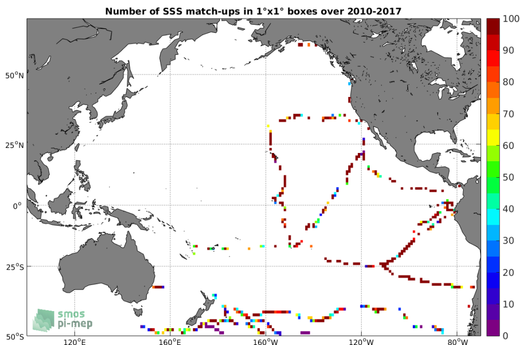
Figure 4: Number of SSS match-ups between TSG-GOSUD-Sailing-ship SSS and the SMOS L2Q v321 - 0.25 Deg (CATDS-CPDC) SSS product for the Pacific Ocean Pi-MEP region over 1°x1° boxes and for the full satellite product period.
