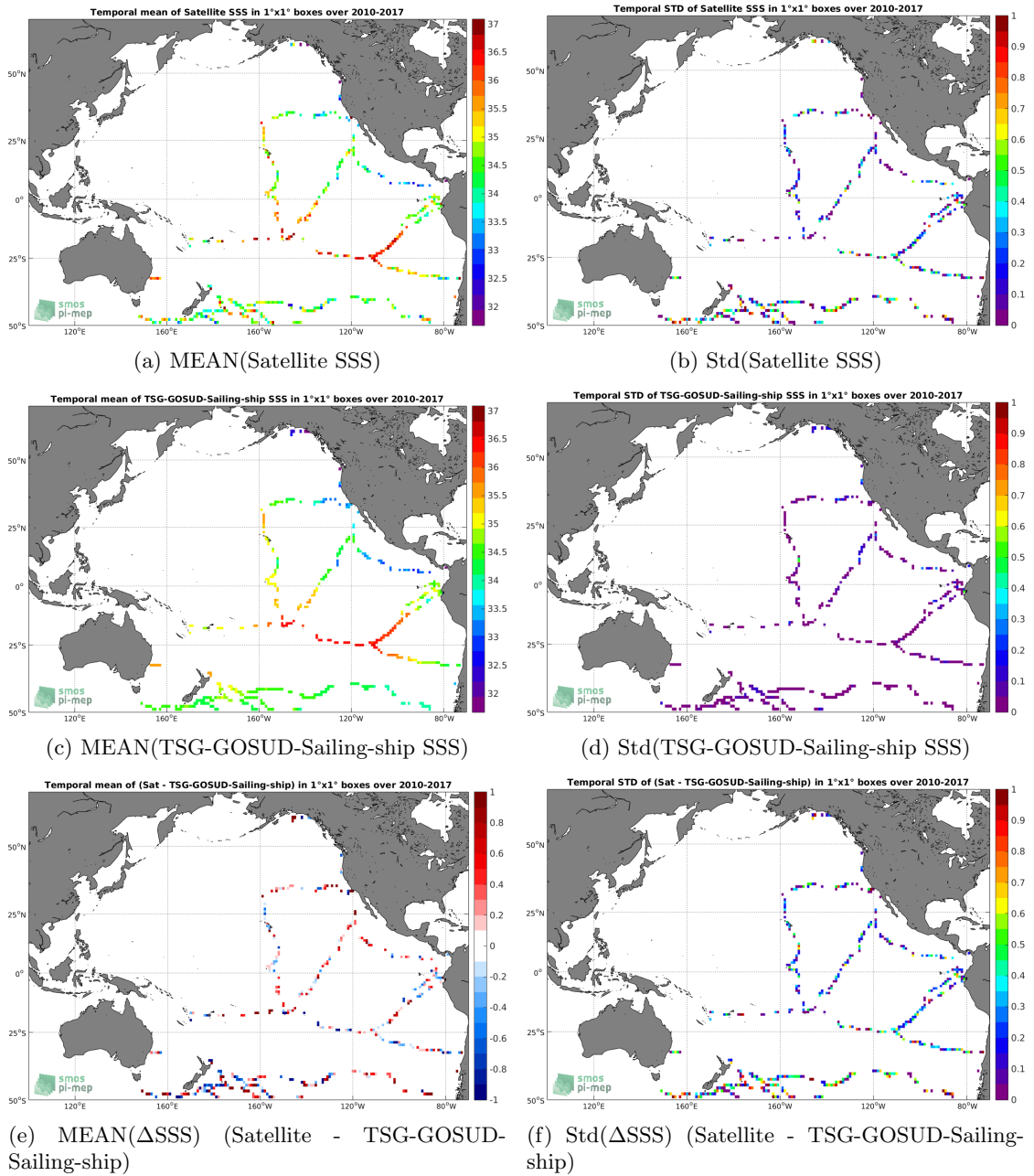
Figure 6: Temporal mean (left) and Std (right) of SSS from SMOS L2Q v321 - 0.25 Deg (CATDS-CPDC) (top), TSG-GOSUD-Sailing-ship (middle), and of \Delta SSS (Satellite - TSG-GOSUD-Sailing-ship). Only match-up pairs are used to generate these maps.
