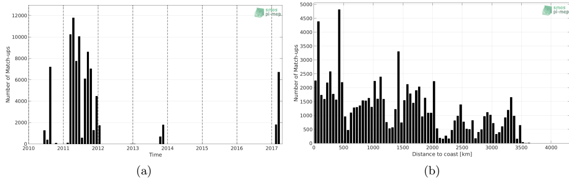
Figure 1: Number of match-ups between TSG-GOSUD-Sailing-ship and SMOS L2Q v321 - 0.25 Deg (CATDS-CPDC) SSS as a function of time (a) and as function of the distance to coast (b) over the Pacific Ocean Pi-MEP region and for the full satellite product period.
