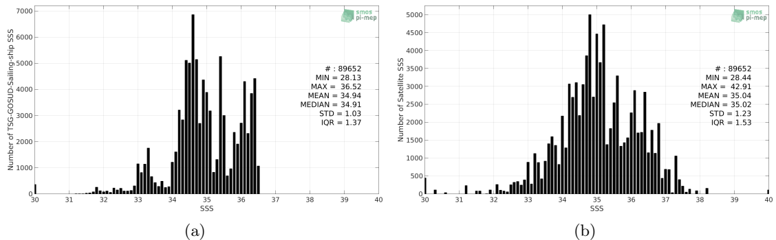
Figure 2: Histograms of SSS from TSG-GOSUD-Sailing-ship (a) and SMOS L2Q v321 - 0.25 Deg (CATDS-CPDC) (b) considering all match-up pairs per bins of 0.1 over the Pacific Ocean Pi-MEP region and for the full satellite product period.
