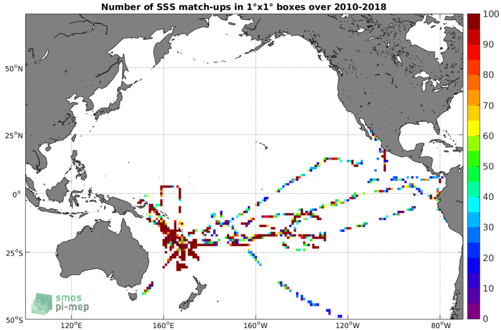
Figure 4: Number of SSS match-ups between TSG-GOSUD-Research-vessel SSS and the SMOS L2Q v321 - 0.25 Deg (CATDS-CPDC) SSS product for the Pacific Ocean Pi-MEP region over 1°x1° boxes and for the full satellite product period.
