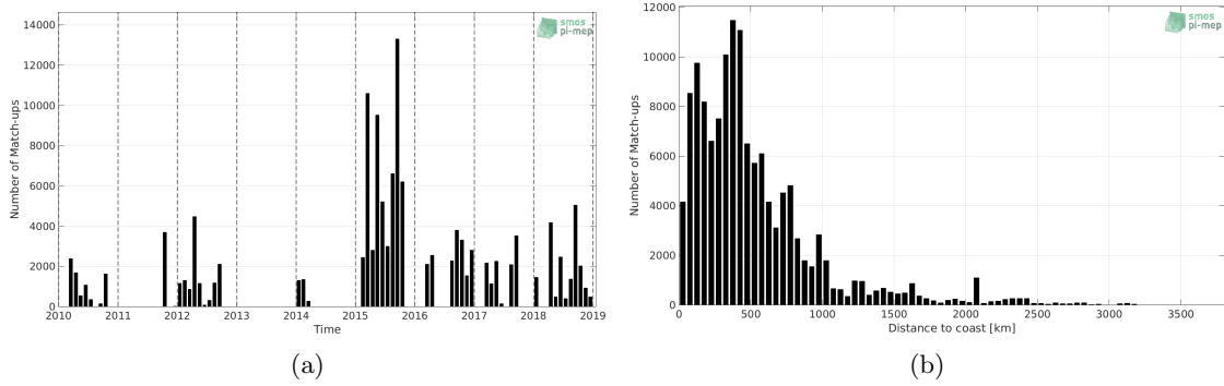
Figure 1: Number of match-ups between TSG-GOSUD-Research-vessel and SMOS L2Q v321 - 0.25 Deg (CATDS-CPDC) SSS as a function of time (a) and as function of the distance to coast (b) over the Pacific Ocean Pi-MEP region and for the full satellite product period.
