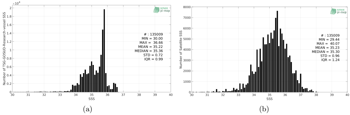
Figure 2: Histograms of SSS from TSG-GOSUD-Research-vessel (a) and SMOS L2Q v321 - 0.25 Deg (CATDS-CPDC) (b) considering all match-up pairs per bins of 0.1 over the Pacific Ocean Pi-MEP region and for the full satellite product period.
