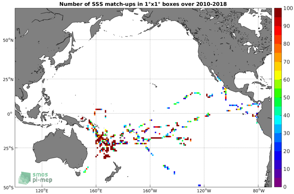
Figure 4: Number of SSS match-ups between TSG-GOSUD-Research-vessel SSS and the SMOS-L3-CATDS-CPDC-V321-L2Q SSS product for the Pacific Ocean Pi-MEP region over 1°x1° boxes and for the full satellite product period.
