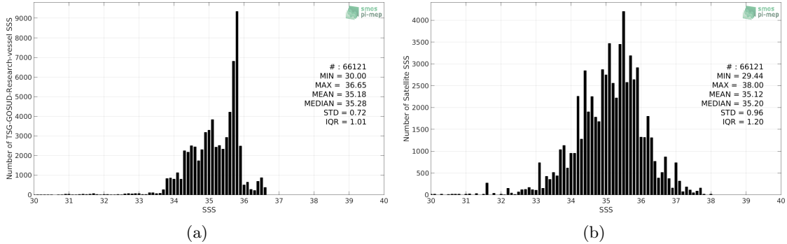
Figure 2: Histograms of SSS from TSG-GOSUD-Research-vessel (a) and SMOS-L3-CATDS-CPDC-V321-L2Q (b) considering all match-up pairs per bins of 0.1 over the Pacific Ocean Pi-MEP region and for the full satellite product period.
