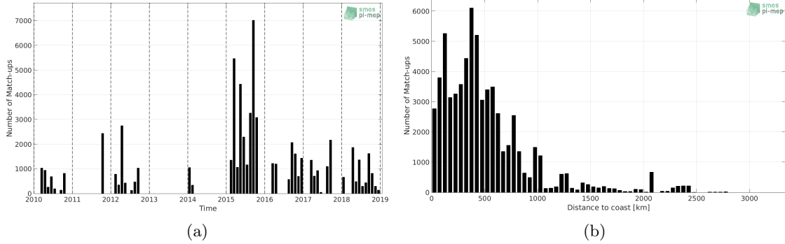
Figure 1: Number of match-ups between TSG-GOSUD-Research-vessel and SMOS-L3-CATDS-CPDC-V321-L2Q SSS as a function of time (a) and as function of the distance to coast (b) over the Pacific Ocean Pi-MEP region and for the full satellite product period.
