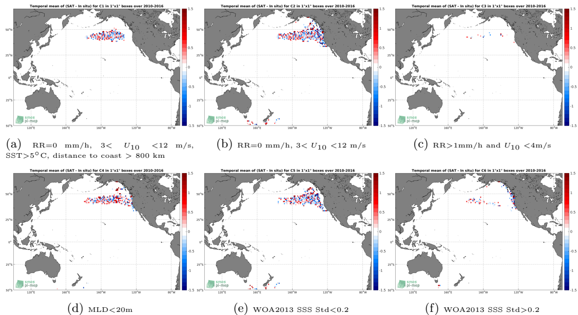
Figure 12: Temporal mean gridded over spatial boxes of size 1^\circ \times 1^\circ of \Delta SSS (SMOS SSS L2Q v321 - 0.25 Deg (CATDS-CPDC) - Marine mammals) for 6 different subdatasets corresponding to:RR=0 mm/h, 3 < U_{10} < 12 m/s, SST > 5^\circ\text{C} , distance to coast > 800 km (a), RR=0 mm/h, 3 < U_{10} < 12 m/s (b), RR > 1 mm/h and U_{10} < 4 m/s (c),MLD < 20 m (d),WOA2013 SSS Std < 0.2 (e),WOA2013 SSS Std > 0.2 (f).
