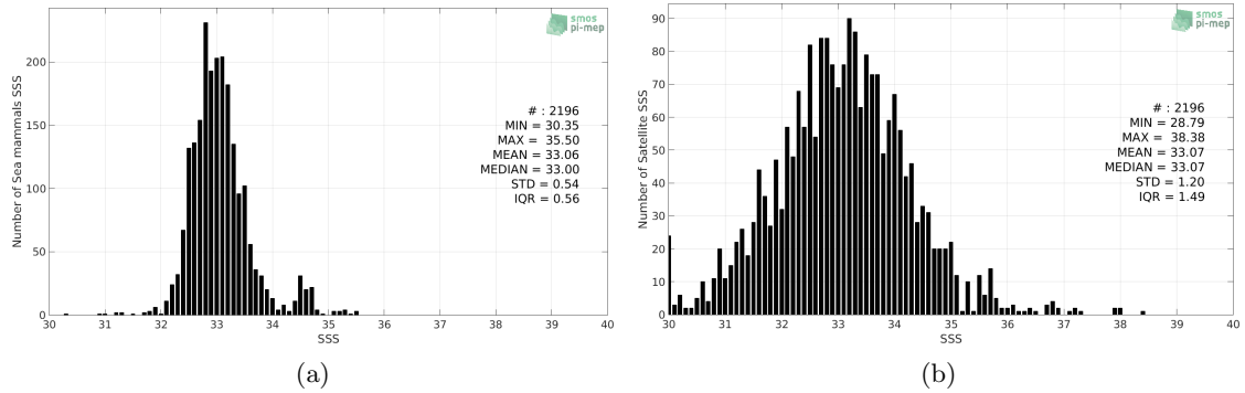
Figure 2: Histograms of SSS from Marine mammals (a) and SMOS SSS L2Q v321 - 0.25 Deg (CATDS-CPDC) (b) considering all match-up pairs per bins of 0.1 over the Pacific Ocean Pi-MEP region and for the full satellite product period.
