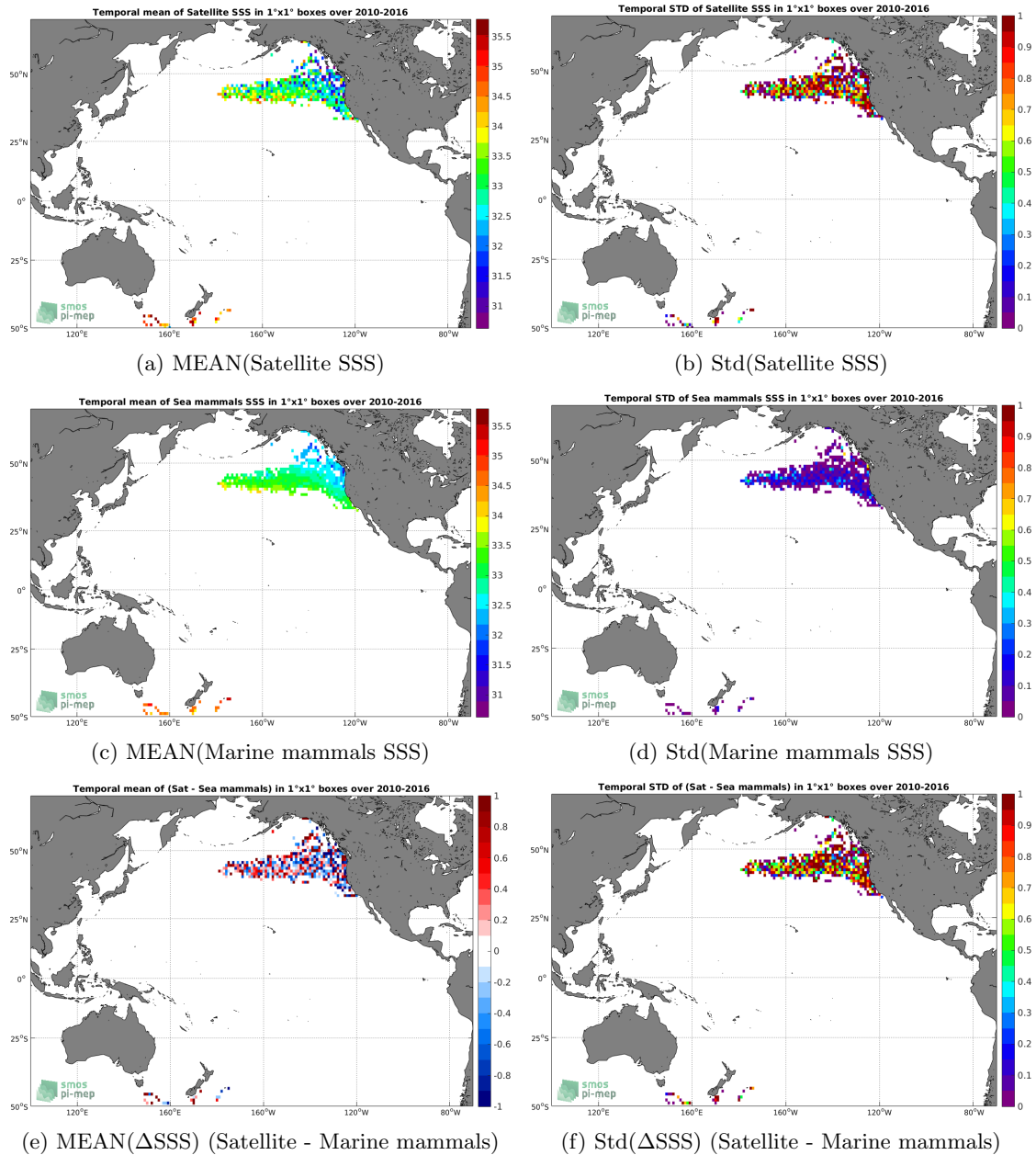
Figure 6: Temporal mean (left) and Std (right) of SSS from SMOS SSS L2Q v321 - 0.25 Deg (CATDS-CPDC) (top), Marine mammals (middle), and of \Delta SSS (Satellite - Marine mammals). Only match-up pairs are used to generate these maps.
