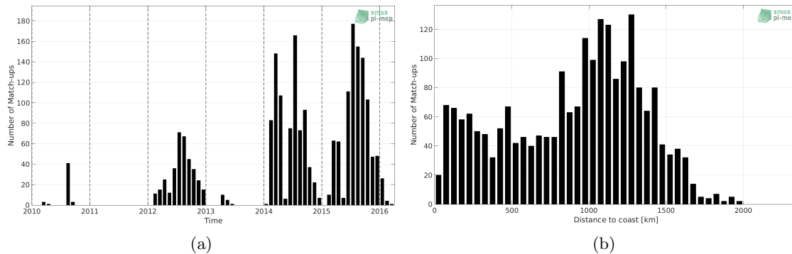
Figure 1: Number of match-ups between Marine mammals and SMOS SSS L2Q v321 - 0.25 Deg (CATDS-CPDC) SSS as a function of time (a) and as function of the distance to coast (b) over the Pacific Ocean Pi-MEP region and for the full satellite product period.
