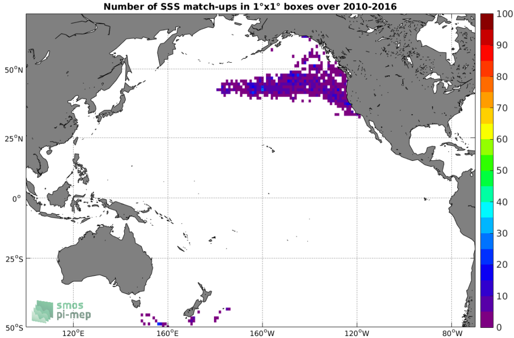
Figure 4: Number of SSS match-ups between Marine mammals SSS and the SMOS SSS L2Q v321 - 0.25 Deg (CATDS-CPDC) SSS product for the Pacific Ocean Pi-MEP region over 1^\circ \times 1^\circ boxes and for the full satellite product period.
