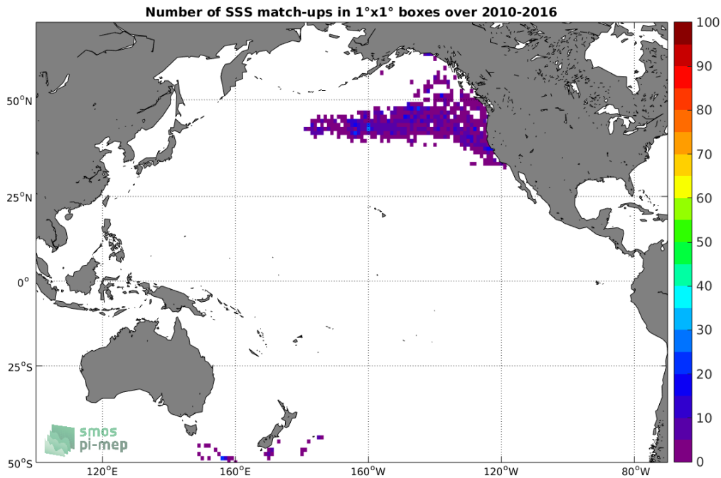
Figure 4: Number of SSS match-ups between Sea mammals SSS and the SMOS L2Q v321 - 0.25 Deg (CATDS-CPDC) SSS product for the Pacific Ocean Pi-MEP region over 1°x1° boxes and for the full satellite product period.
