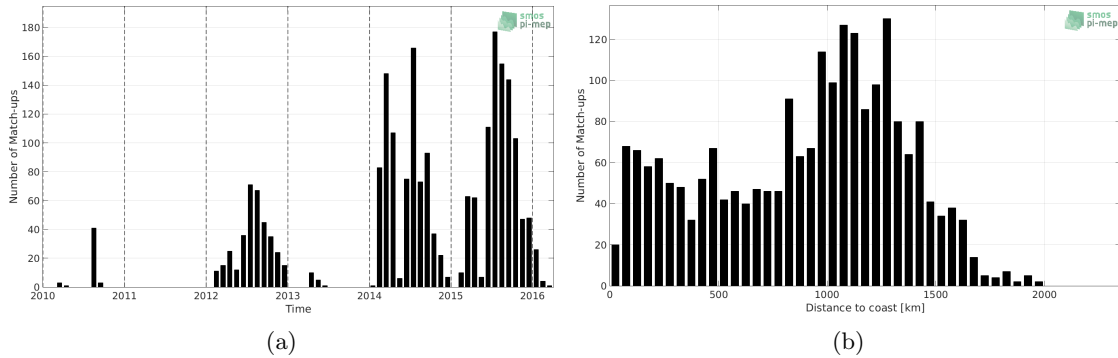
Figure 1: Number of match-ups between Sea mammals and SMOS L2Q v321 - 0.25 Deg (CATDS-CPDC) SSS as a function of time (a) and as function of the distance to coast (b) over the Pacific Ocean Pi-MEP region and for the full satellite product period.
