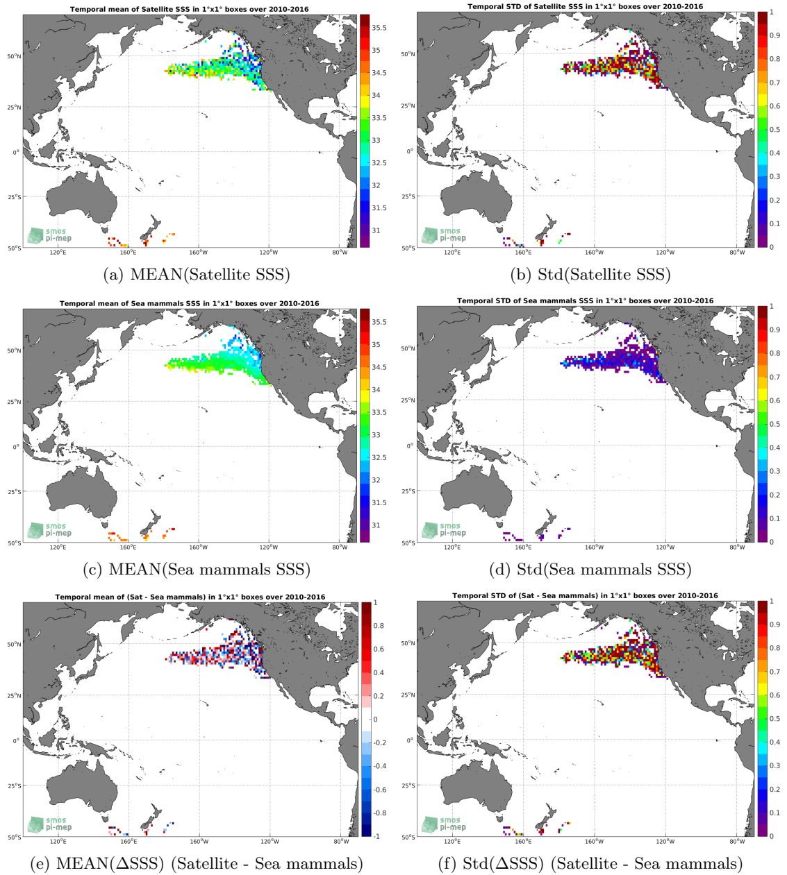
Figure 6: Temporal mean (left) and Std (right) of SSS from SMOS L2Q v321 - 0.25 Deg (CATDS-CPDC) (top), Sea mammals (middle), and of \Delta SSS (Satellite - Sea mammals). Only match-up pairs are used to generate these maps.
