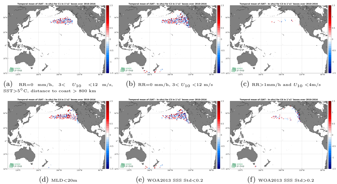
Figure 12: Temporal mean gridded over spatial boxes of size 1^\circ \times 1^\circ of \Delta SSS (SMOS L2Q v321 - 0.25 Deg (CATDS-CPDC) - Sea mammals) for 6 different subdatasets corresponding to:RR=0 mm/h, 3 < U_{10} < 12 m/s, SST > 5^\circ\text{C} , distance to coast > 800 km (a), RR=0 mm/h, 3 < U_{10} < 12 m/s (b), RR > 1 mm/h and U_{10} < 4 m/s (c),MLD < 20 m (d),WOA2013 SSS Std < 0.2 (e),WOA2013 SSS Std > 0.2 (f).
