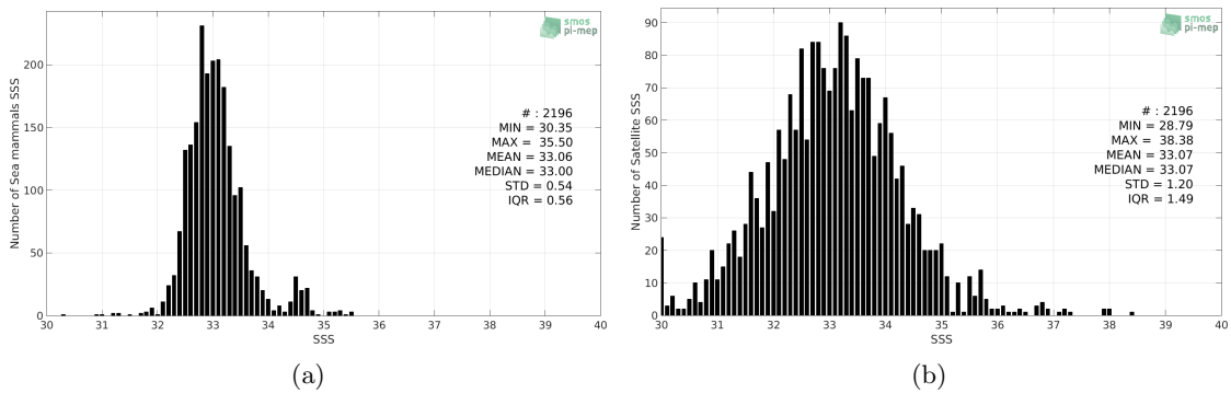
Figure 2: Histograms of SSS from Sea mammals (a) and SMOS L2Q v321 - 0.25 Deg (CATDS-CPDC) (b) considering all match-up pairs per bins of 0.1 over the Pacific Ocean Pi-MEP region and for the full satellite product period.
