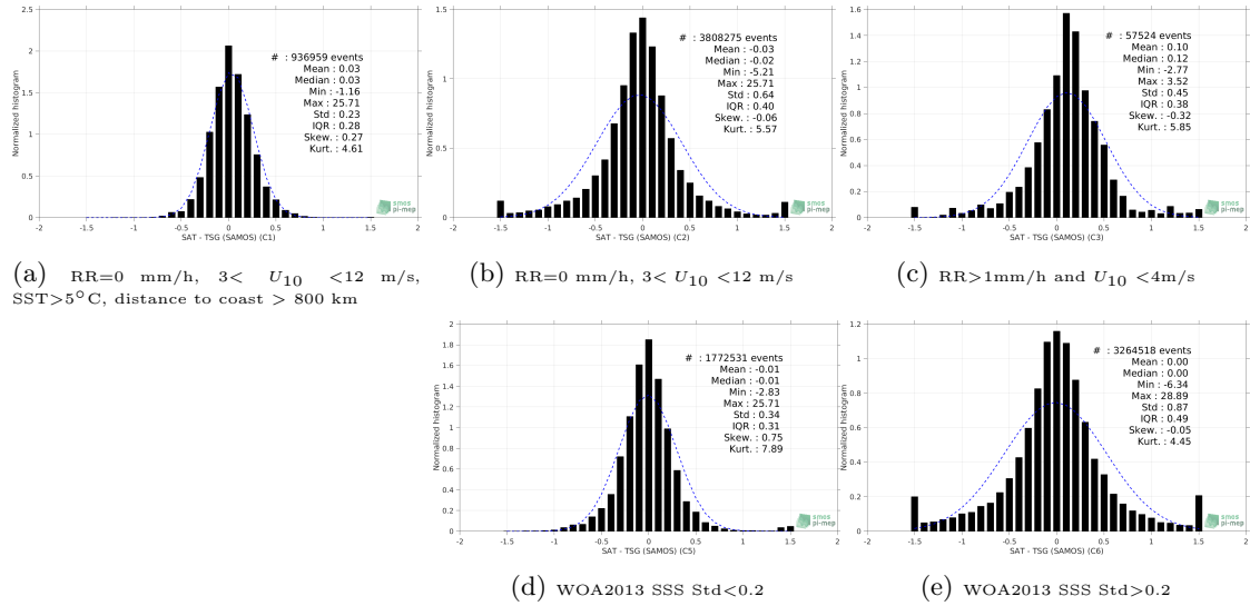
Figure 13: Normalized histogram of \Delta\text{SSS} (SMOS SSS L3 v317 - Monthly - 25 km (CATDS-CPDC) - TSG (SAMOS)) for 5 different subdatasets corresponding to: RR=0 mm/h, 3 < U_{10} < 12 m/s, SST>5°C, distance to coast > 800 km (a), RR=0 mm/h, 3 < U_{10} < 12 m/s (b), RR>1mm/h and U_{10} < 4 m/s (c), WOA2013 SSS Std<0.2 (d), WOA2013 SSS Std>0.2 (e).
