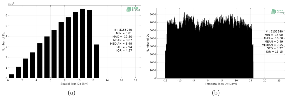
Figure 5: Histograms of the spatial (a) and temporal (b) lags between the location/time of the TSG (SAMOS) measurement and the date of the corresponding SMOS SSS L3 v317 - Monthly - 25 km (CATDS-CPDC) SSS pixel.
