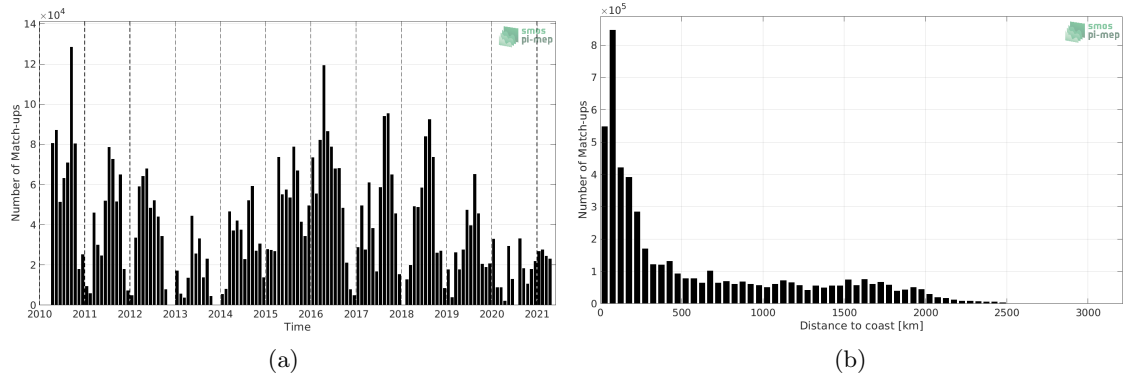
Figure 1: Number of match-ups between TSG (SAMOS) and SMOS SSS L3 v317 - Monthly - 25 km (CATDS-CPDC) SSS as a function of time (a) and as function of the distance to coast (b) over the Pacific Ocean Pi-MEP region and for the full satellite product period.
