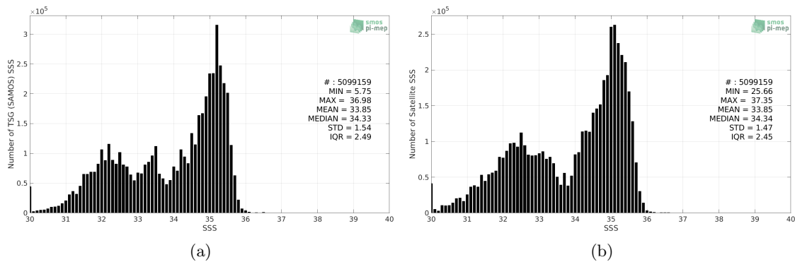
Figure 2: Histograms of SSS from TSG (SAMOS) (a) and SMOS SSS L3 v317 - Monthly - 25 km (CATDS-CPDC) (b) considering all match-up pairs per bins of 0.1 over the Pacific Ocean Pi-MEP region and for the full satellite product period.
