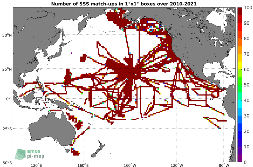
Figure 4: Number of SSS match-ups between TSG (SAMOS) SSS and the SMOS SSS L3 v317 - Monthly - 25 km (CATDS-CPDC) SSS product for the Pacific Ocean Pi-MEP region over 1^\circ \times 1^\circ boxes and for the full satellite product period.
