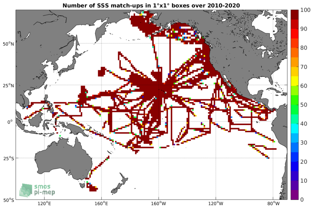
Figure 4: Number of SSS match-ups between TSG-SAMOS SSS and the SMOS L3 v317 - Monthly - 25 km (CATDS-CPDC) SSS product for the Pacific Ocean Pi-MEP region over 1°x1° boxes and for the full satellite product period.
