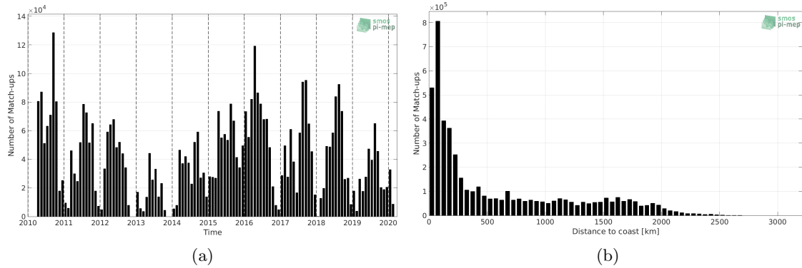
Figure 1: Number of match-ups between TSG-SAMOS and SMOS L3 v317 - Monthly - 25 km (CATDS-CPDC) SSS as a function of time (a) and as function of the distance to coast (b) over the Pacific Ocean Pi-MEP region and for the full satellite product period.
