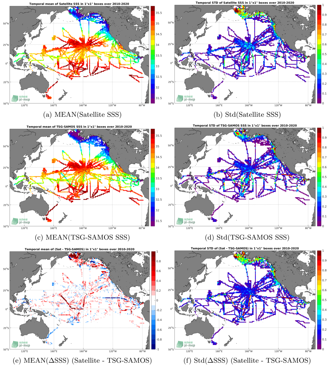
Figure 6: Temporal mean (left) and Std (right) of SSS from SMOS L3 v317 - Monthly - 25 km (CATDS-CPDC) (top), TSG-SAMOS (middle), and of \Delta SSS (Satellite - TSG-SAMOS). Only match-up pairs are used to generate these maps.
