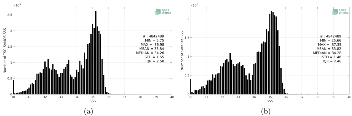
Figure 2: Histograms of SSS from TSG-SAMOS (a) and SMOS L3 v317 - Monthly - 25 km (CATDS-CPDC) (b) considering all match-up pairs per bins of 0.1 over the Pacific Ocean Pi-MEP region and for the full satellite product period.
