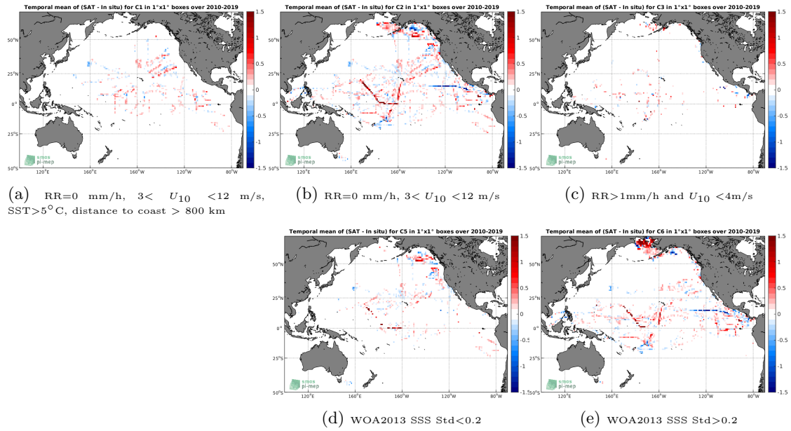
Figure 12: Temporal mean gridded over spatial boxes of size 1^\circ \times 1^\circ of \Delta SSS (SMOS-L3-CATDS-CPDC-V317-MONTHLY-25KM - TSG-SAMOS) for 5 different subdatasets corresponding to: RR=0 mm/h, 3 < U_{10} < 12 m/s, SST > 5^\circ\text{C} , distance to coast > 800 km (a), RR=0 mm/h, 3 < U_{10} < 12 m/s (b), RR > 1 mm/h and U_{10} < 4 m/s (c), WOA2013 SSS Std < 0.2 (d), WOA2013 SSS Std > 0.2 (e).
