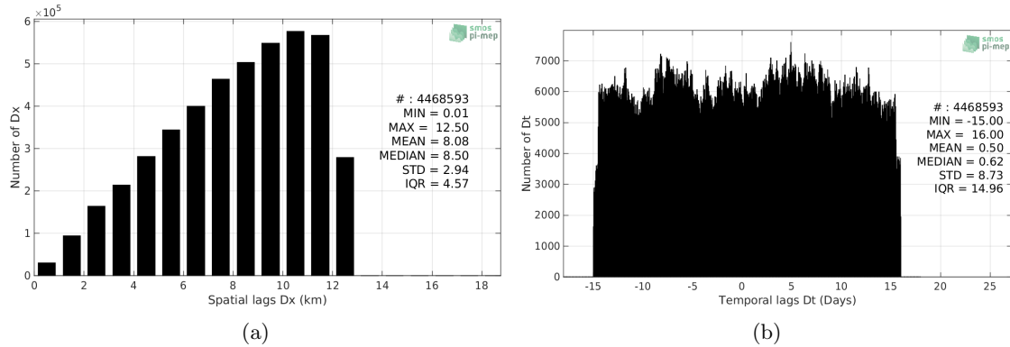
Figure 5: Histograms of the spatial (a) and temporal (b) lags between the time of the TSG-SAMOS measurements and the date of the corresponding SMOS-L3-CATDS-CPDC-V317-MONTHLY-25KM SSS product.
