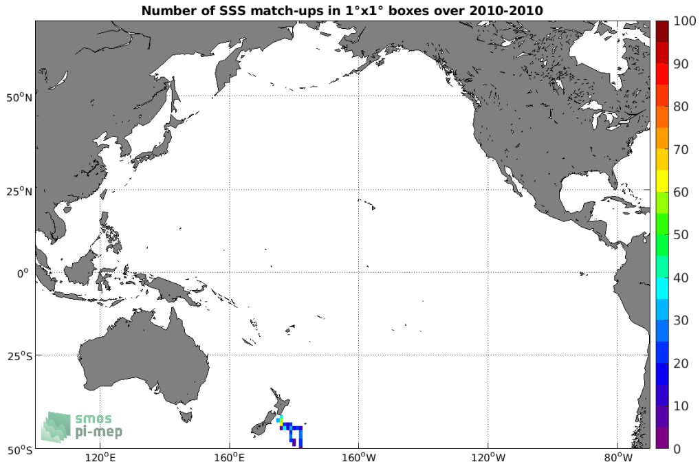
Figure 4: Number of SSS match-ups between TSG (Polarstern) SSS and the SMOS SSS L3 v317 - Monthly - 25 km (CATDS-CPDC) SSS product for the Pacific Ocean Pi-MEP region over 1°x1° boxes and for the full satellite product period.
