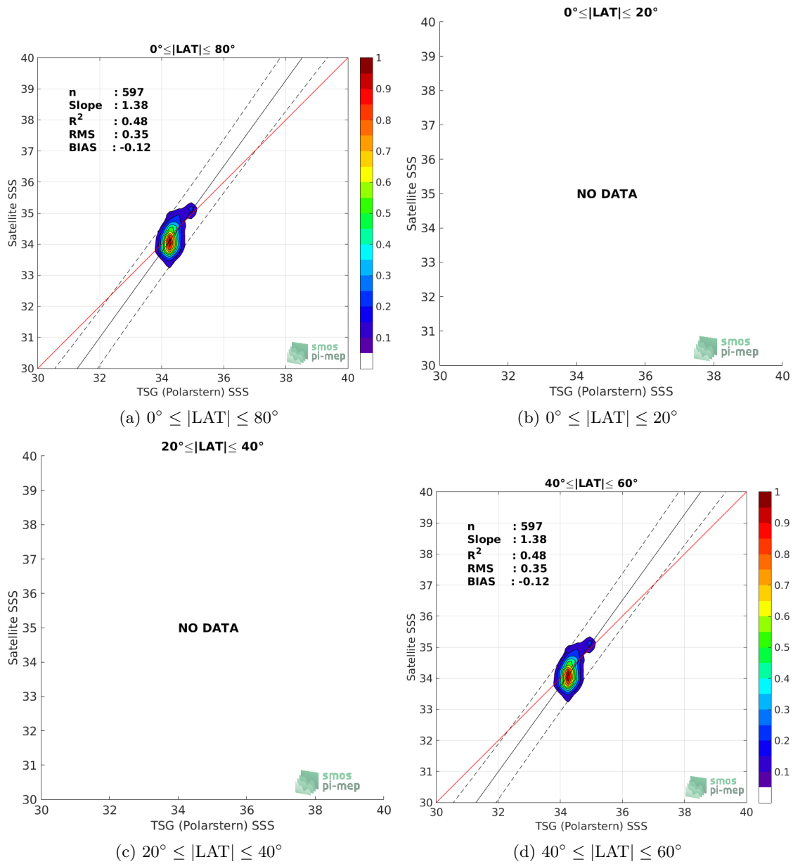
Figure 9: Contour maps of the concentration of SMOS SSS L3 v317 - Monthly - 25 km (CATDS-CPDC) SSS ( y -axis) versus TSG (Polarstern) SSS ( x -axis) at match-up pairs for different latitude bands. For each plot, the red line shows x=y . The black thin and dashed lines indicate a linear fit through the data cloud and the \pm 95\% confidence levels, respectively. The number match-up pairs n , the slope and R^2 coefficient of the linear fit, the root mean square (RMS) and the mean bias between satellite and in situ data are indicated for each latitude band in each plots.
