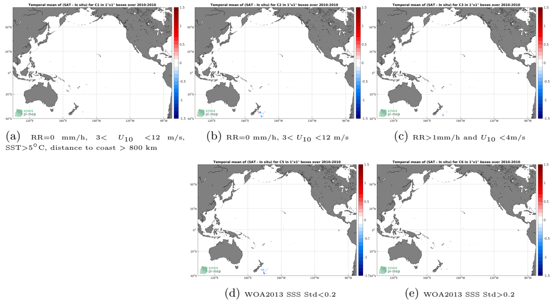
Figure 12: Temporal mean gridded over spatial boxes of size 1^\circ \times 1^\circ of \Delta SSS (SMOS-L3-CATDS-CPDC-V317-MONTHLY-25KM - TSG-POLARSTERN) for 5 different subdatasets corresponding to:RR=0 mm/h, 3 < U_{10} < 12 m/s, SST >5^\circ C, distance to coast > 800 km (a), RR=0 mm/h, 3 < U_{10} < 12 m/s (b), RR >1 mm/h and U_{10} < 4 m/s (c), WOA2013 SSS Std <0.2 (d), WOA2013 SSS Std >0.2 (e).
