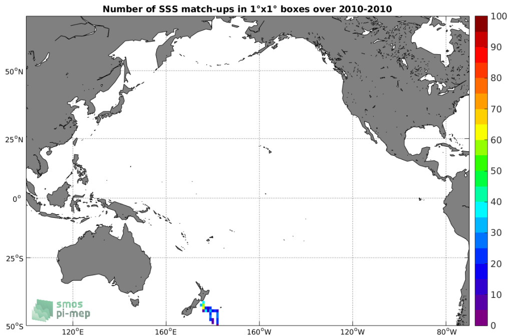
Figure 4: Number of SSS match-ups between TSG-POLARSTERN SSS and the SMOS-L3-CATDS-CPDC-V317-MONTHLY-25KM SSS product for the Pacific Ocean Pi-MEP region over 1^\circ \times 1^\circ boxes and for the full satellite product period.
