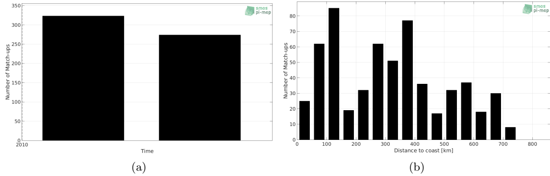
Figure 1: Number of match-ups between TSG-POLARSTERN and SMOS-L3-CATDS-CPDC-V317-MONTHLY-25KM SSS as a function of time (a) and as function of the distance to coast (b) over the Pacific Ocean Pi-MEP region and for the full satellite product period.
