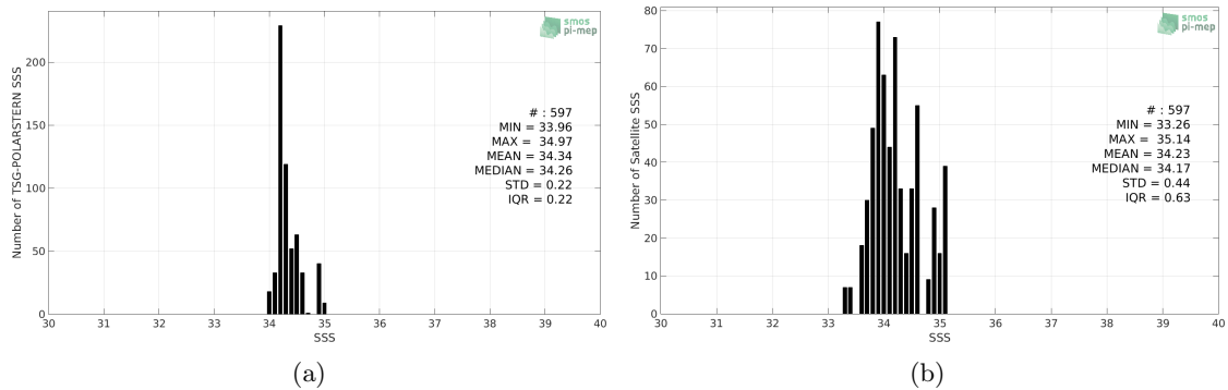
Figure 2: Histograms of SSS from TSG-POLARSTERN (a) and SMOS-L3-CATDS-CPDC-V317-MONTHLY-25KM (b) considering all match-up pairs per bins of 0.1 over the Pacific Ocean Pi-MEP region and for the full satellite product period.
