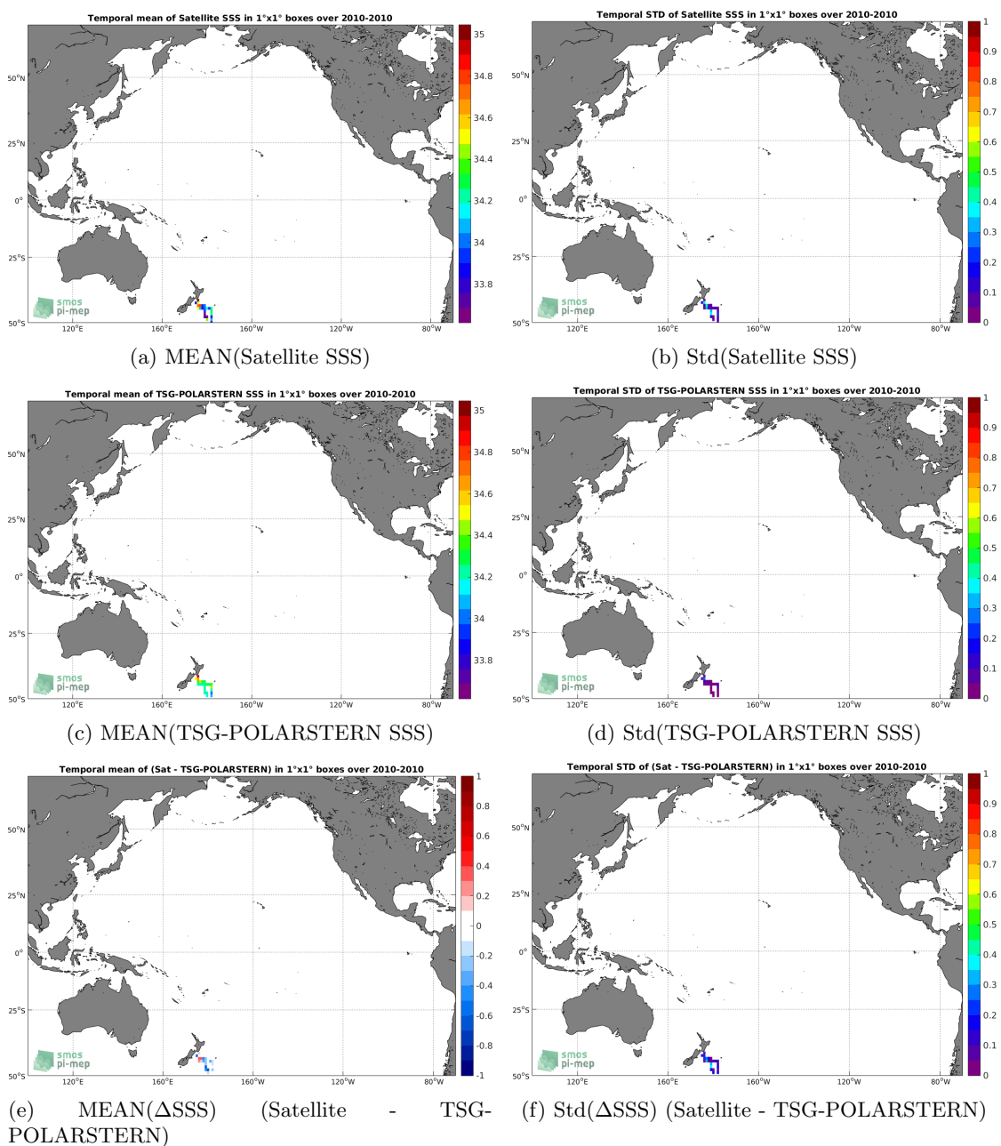
Figure 6: Temporal mean (left) and Std (right) of SSS from SMOS-L3-CATDS-CPDC-V317-MONTHLY-25KM (top), TSG-POLARSTERN (middle), and of \Delta SSS (Satellite - TSG-POLARSTERN). Only match-up pairs are used to generate these maps.
