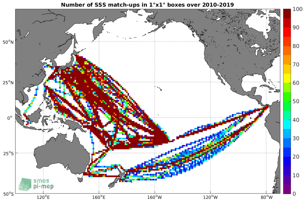
Figure 4: Number of SSS match-ups between TSG (LEGOS-DM) SSS and the SMOS SSS L3 v317 - Monthly - 25 km (CATDS-CPDC) SSS product for the Pacific Ocean Pi-MEP region over 1°x1° boxes and for the full satellite product period.
