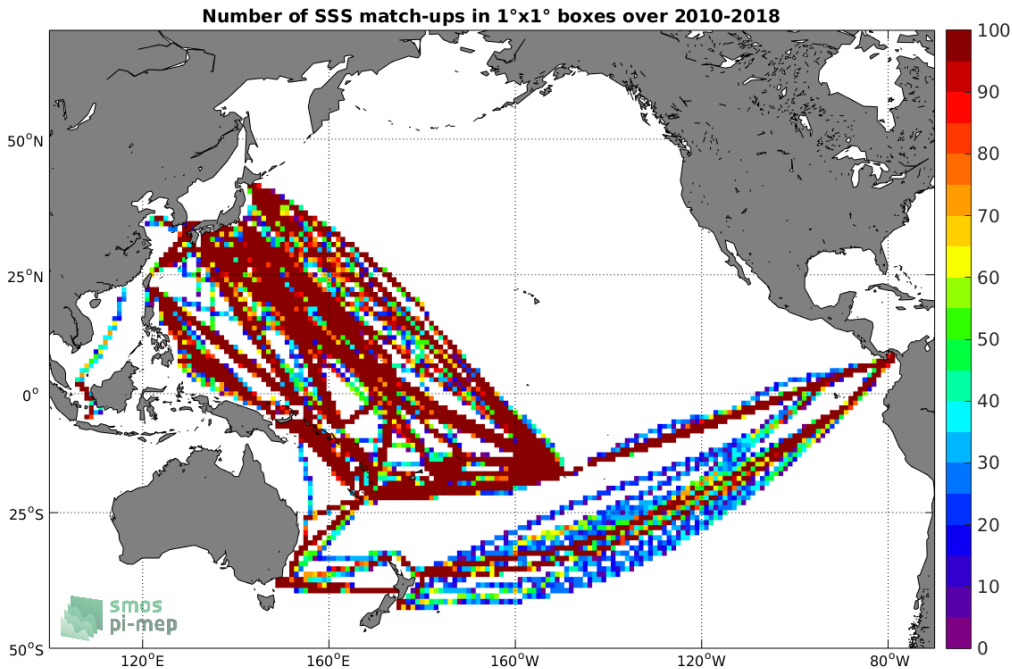
Figure 4: Number of SSS match-ups between TSG-LEGOS-DM SSS and the SMOS-L3-CATDS-CPDC-V317-MONTHLY-25KM SSS product for the Pacific Ocean Pi-MEP region over 1°x1° boxes and for the full satellite product period.
