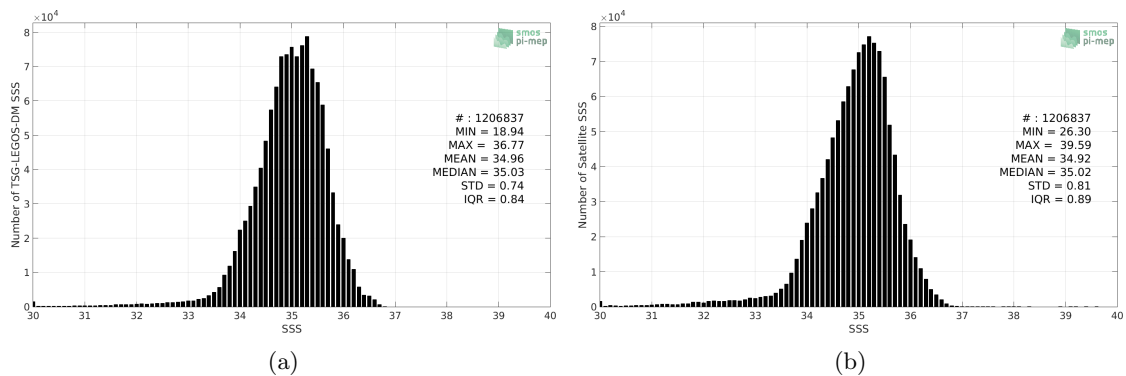
Figure 2: Histograms of SSS from TSG-LEGOS-DM (a) and SMOS-L3-CATDS-CPDC-V317-MONTHLY-25KM (b) considering all match-up pairs per bins of 0.1 over the Pacific Ocean Pi-MEP region and for the full satellite product period.
