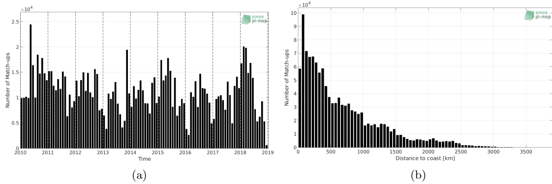
Figure 1: Number of match-ups between TSG-LEGOS-DM and SMOS-L3-CATDS-CPDC-V317-MONTHLY-25KM SSS as a function of time (a) and as function of the distance to coast (b) over the Pacific Ocean Pi-MEP region and for the full satellite product period.
