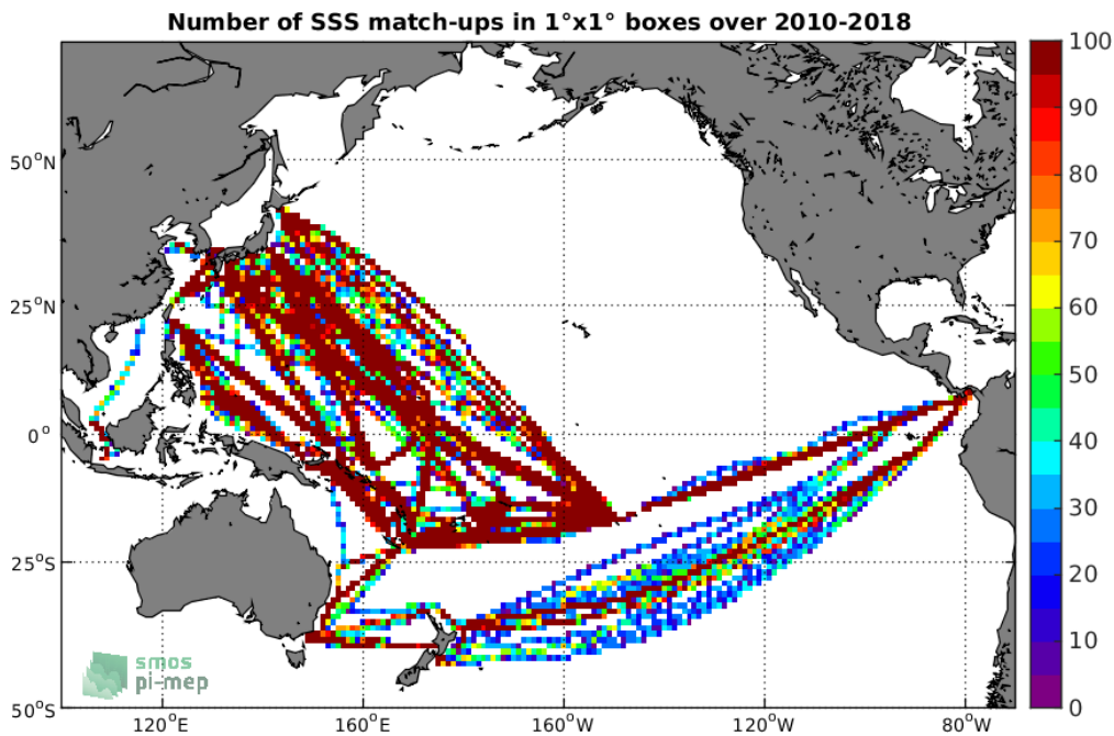
Figure 4: Number of SSS match-ups between TSG-LEGOS-DM SSS and the SMOS-L3-CATDS-CPDC-V317-MONTHLY-25KM SSS product for the Pacific Ocean Pi-MEP region over 1^\circ \times 1^\circ boxes and for the full satellite product period.
