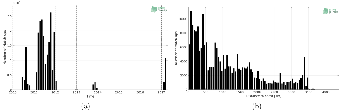
Figure 1: Number of match-ups between TSG-GOSUD-Sailing-ship and SMOS-L3-CATDS-CPDC-V317-MONTHLY-25KM SSS as a function of time (a) and as function of the distance to coast (b) over the Pacific Ocean Pi-MEP region and for the full satellite product period.
