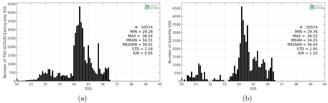
Figure 2: Histograms of SSS from TSG-GOSUD-Sailing-ship (a) and SMOS-L3-CATDS-CPDC-V317-MONTHLY-25KM (b) considering all match-up pairs per bins of 0.1 over the Pacific Ocean Pi-MEP region and for the full satellite product period.
