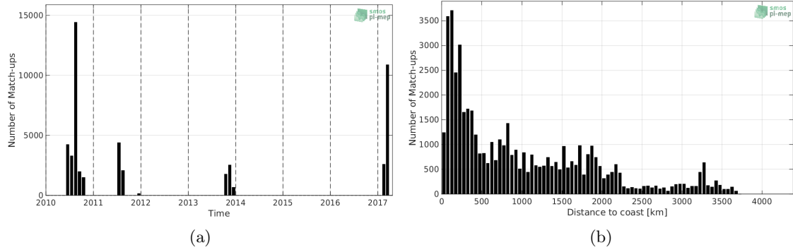
Figure 1: Number of match-ups between TSG-GOSUD-Sailing-ship and SMOS-L3-CATDS-CPDC-V317-MONTHLY-25KM SSS as a function of time (a) and as function of the distance to coast (b) over the Pacific Ocean Pi-MEP region and for the full satellite product period.
