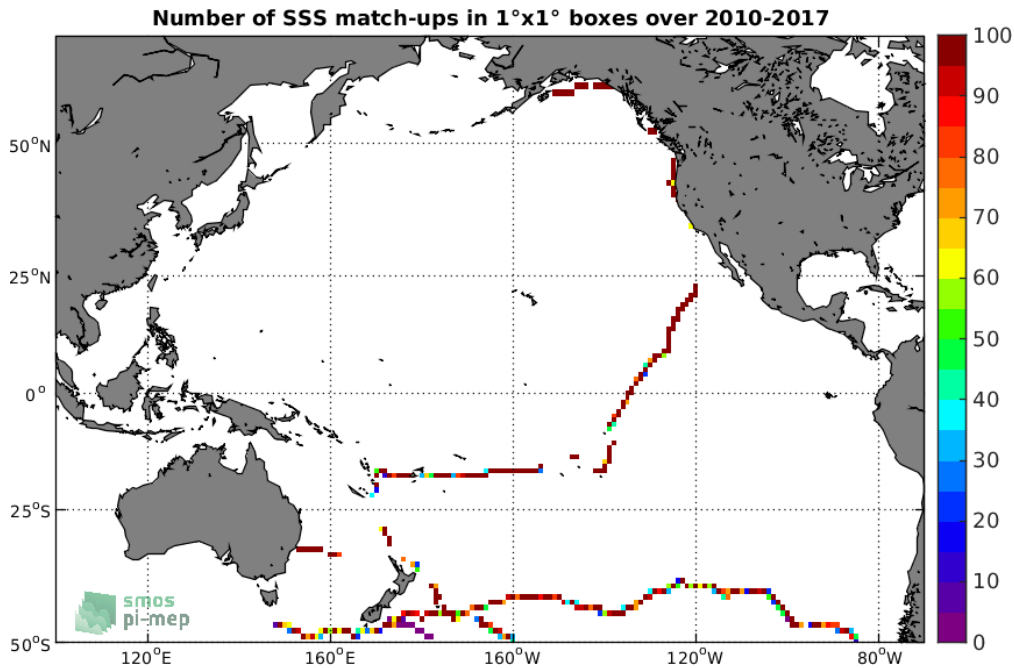
Figure 4: Number of SSS match-ups between TSG-GOSUD-Sailing-ship SSS and the SMOS-L3-CATDS-CPDC-V317-MONTHLY-25KM SSS product for the Pacific Ocean Pi-MEP region over 1^\circ \times 1^\circ boxes and for the full satellite product period.
