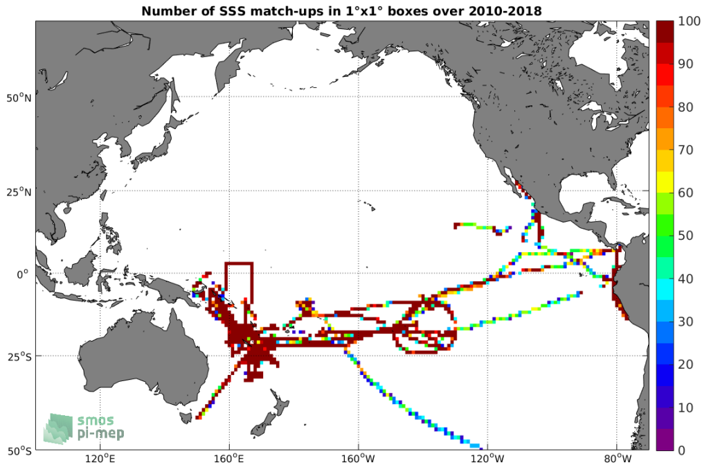
Figure 4: Number of SSS match-ups between TSG (GOSUD-Research-vessel) SSS and the SMOS SSS L3 v317 - Monthly - 25 km (CATDS-CPDC) SSS product for the Pacific Ocean Pi-MEP region over 1°x1° boxes and for the full satellite product period.
