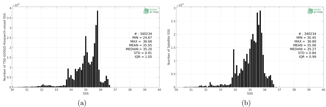
Figure 2: Histograms of SSS from TSG-GOSUD-Research-vessel (a) and SMOS L3 v317 - Monthly - 25 km (CATDS-CPDC) (b) considering all match-up pairs per bins of 0.1 over the Pacific Ocean Pi-MEP region and for the full satellite product period.
