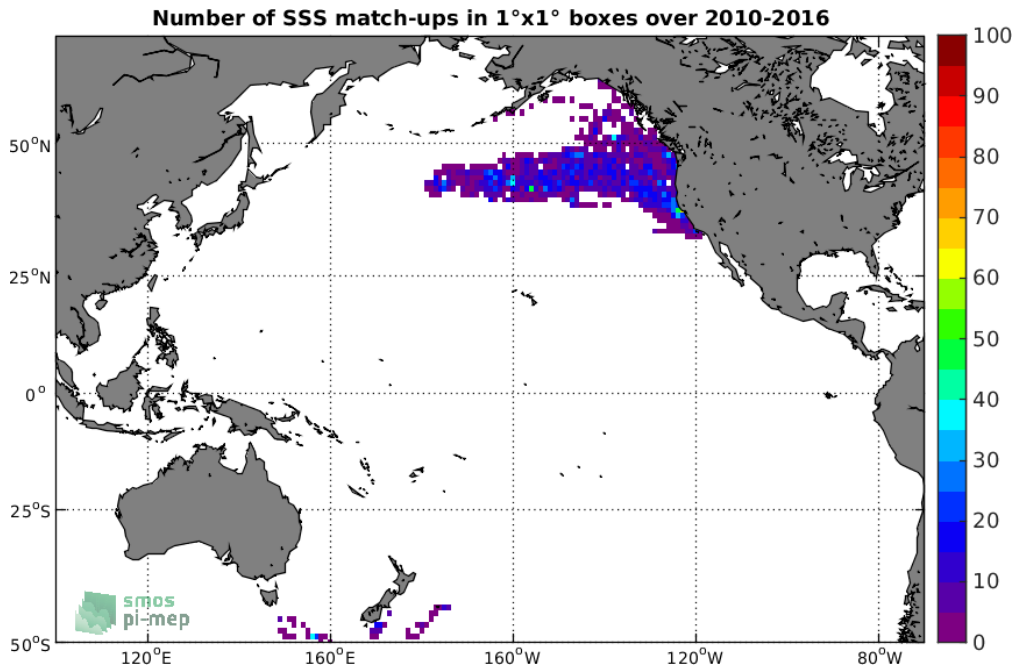
Figure 4: Number of SSS match-ups between Sea mammals SSS and the SMOS-L3-CATDS-CPDC-V317-MONTHLY-25KM SSS product for the Pacific Ocean Pi-MEP region over 1^{\circ} \times 1^{\circ} boxes and for the full satellite product period.
