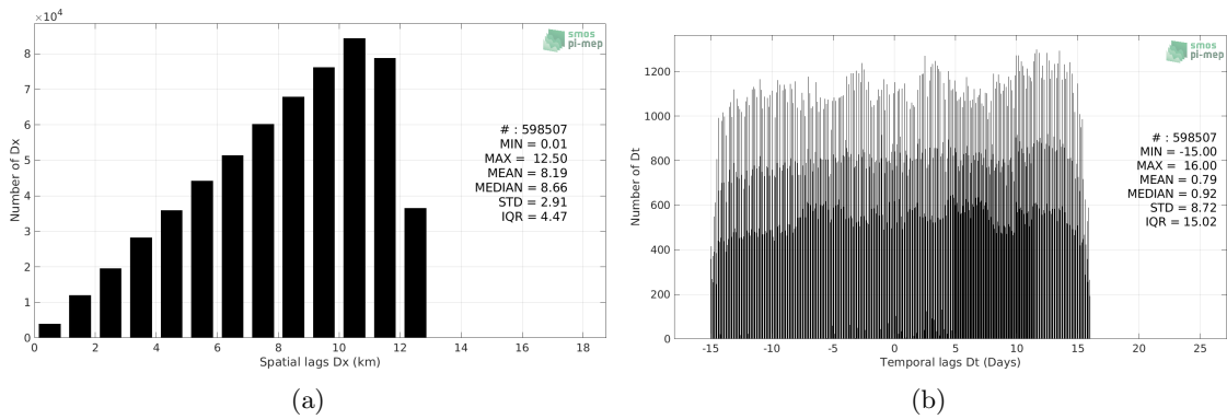
Figure 4: Histograms of the spatial (a) and temporal (b) lags between the location/time of the Surface drifters measurement and the date of the corresponding SMOS SSS L3 v317 - Monthly - 25 km (CATDS-CPDC) SSS pixel.
