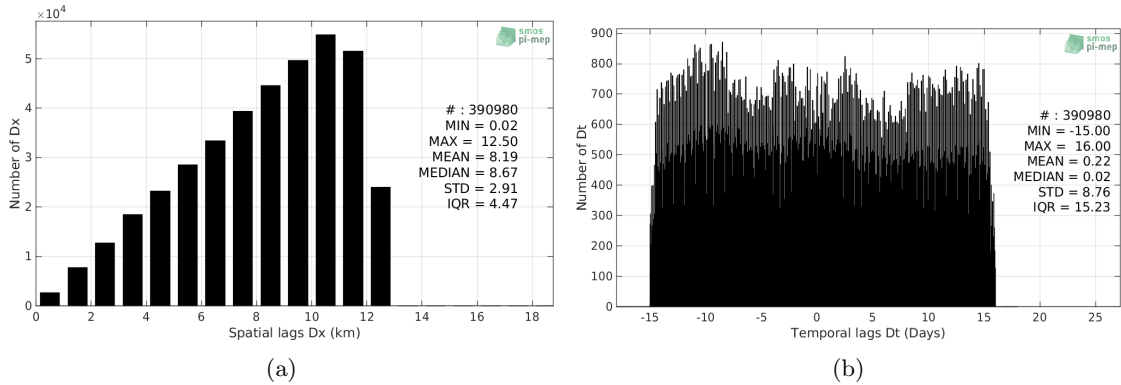
Figure 4: Histograms of the spatial (a) and temporal (b) lags between the time of the Surface drifters measurements and the date of the corresponding SMOS-L3-CATDS-CPDC-V317-MONTHLY-25KM SSS product.
