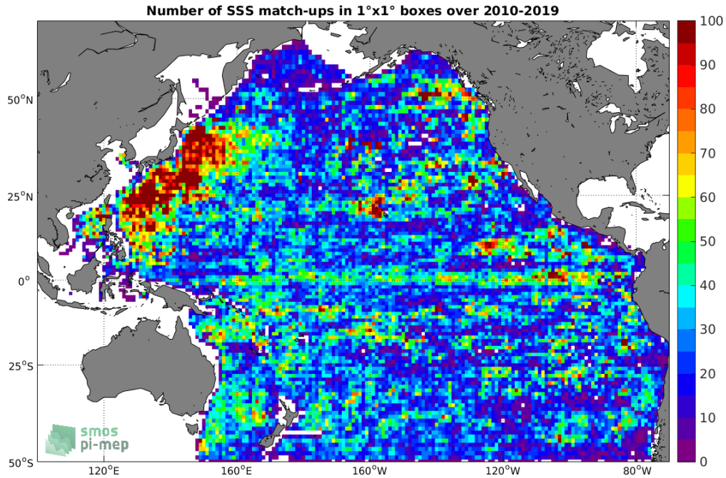
Figure 4: Number of SSS match-ups between Argo SSS and the SMOS-L3-CATDS-CPDC-V317-MONTHLY-25KM SSS product for the Pacific Ocean Pi-MEP region over 1^\circ \times 1^\circ boxes and for the full satellite product period.
