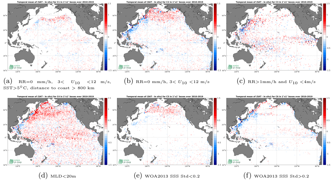
Figure 12: Temporal mean gridded over spatial boxes of size 1^\circ \times 1^\circ of \Delta SSS (SMOS-L3-CATDS-CPDC-V317-MONTHLY-25KM - Argo) for 6 different subdatasets corresponding to: RR=0 mm/h, 3 < U_{10} < 12 m/s, SST > 5^\circ C , distance to coast > 800 km (a), RR=0 mm/h, 3 < U_{10} < 12 m/s (b), RR > 1 mm/h and U_{10} < 4 m/s (c), MLD < 20 m (d), WOA2013 SSS Std < 0.2 (e), WOA2013 SSS Std > 0.2 (f).
