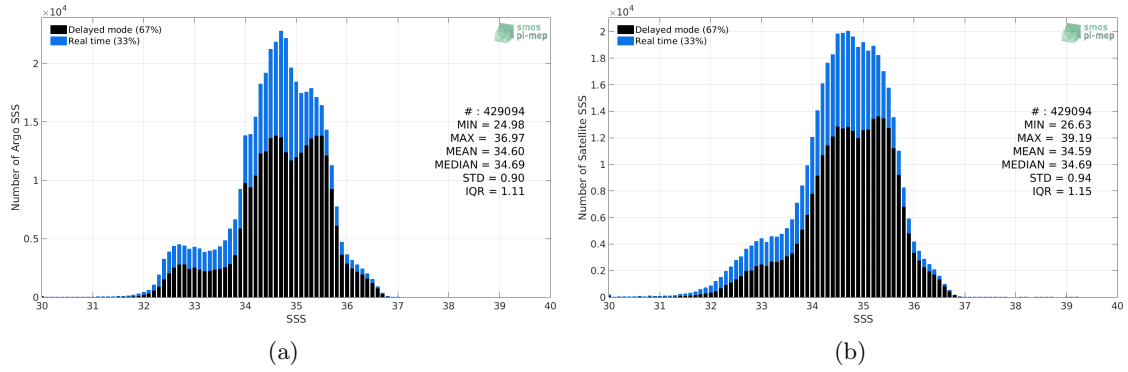
Figure 2: Histograms of SSS from Argo (a) and SMOS-L3-CATDS-CPDC-V317-MONTHLY-25KM (b) considering all match-up pairs per bins of 0.1 over the Pacific Ocean Pi-MEP region and for the full satellite product period.
