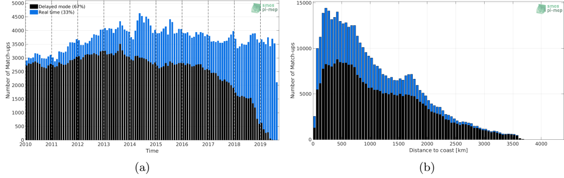
Figure 1: Number of match-ups between Argo and SMOS-L3-CATDS-CPDC-V317-MONTHLY-25KM SSS as a function of time (a) and as function of the distance to coast (b) over the Pacific Ocean Pi-MEP region and for the full satellite product period.
