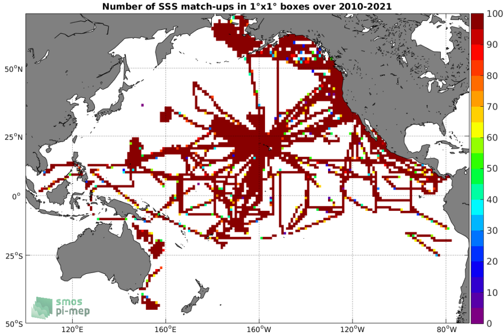
Figure 4: Number of SSS match-ups between TSG (SAMOS) SSS and the SMOS SSS L3 v317 - 10 Days - 25 km (CATDS-CPDC) SSS product for the Pacific Ocean Pi-MEP region over 1°x1° boxes and for the full satellite product period.
