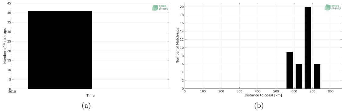
Figure 1: Number of match-ups between TSG (Polarstern) and SMOS SSS L3 v317 - 10 Days - 25 km (CATDS-CPDC) SSS as a function of time (a) and as function of the distance to coast (b) over the Pacific Ocean Pi-MEP region and for the full satellite product period.
