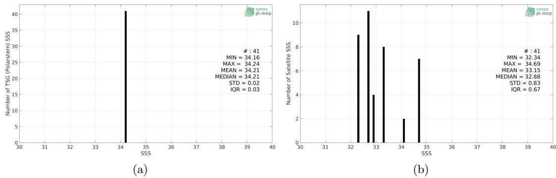
Figure 2: Histograms of SSS from TSG (Polarstern) (a) and SMOS SSS L3 v317 - 10 Days - 25 km (CATDS-CPDC) (b) considering all match-up pairs per bins of 0.1 over the Pacific Ocean Pi-MEP region and for the full satellite product period.
