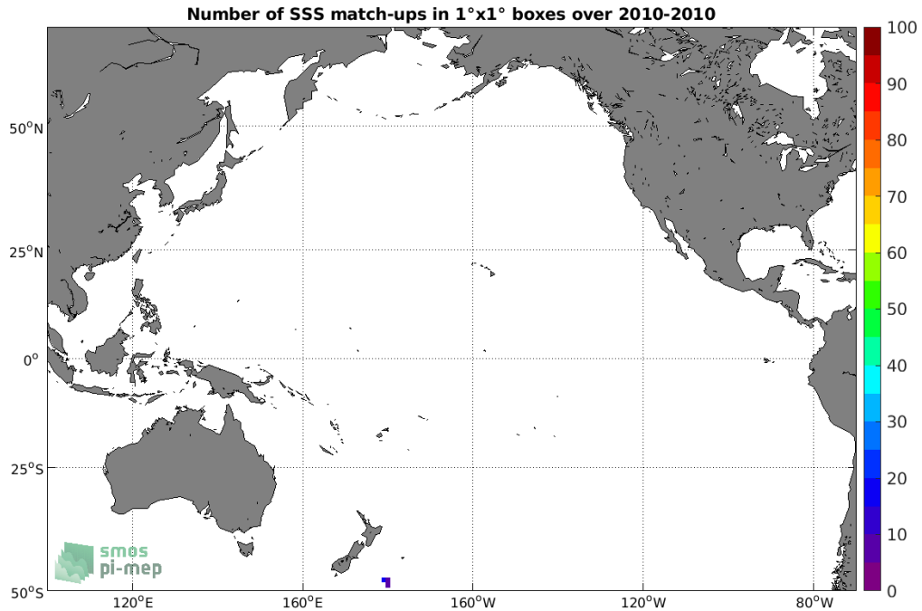
Figure 4: Number of SSS match-ups between TSG (Polarstern) SSS and the SMOS SSS L3 v317 - 10 Days - 25 km (CATDS-CPDC) SSS product for the Pacific Ocean Pi-MEP region over 1^\circ \times 1^\circ boxes and for the full satellite product period.
