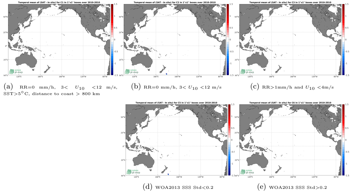
Figure 12: Temporal mean gridded over spatial boxes of size 1^{\circ}\times 1^{\circ} of \Delta\text{SSS} (SMOS SSS L3 v317 - 10 Days - 25 km (CATDS-CPDC) - TSG (Polarstern)) for 5 different subdatasets corresponding to:RR=0 mm/h, 3 < U_{10} < 12 m/s, SST > 5^{\circ}\text{C} , distance to coast > 800 km (a), RR=0 mm/h, 3 < U_{10} < 12 m/s (b), RR > 1 mm/h and U_{10} < 4 m/s (c), WOA2013 SSS Std < 0.2 (d), WOA2013 SSS Std > 0.2 (e).
