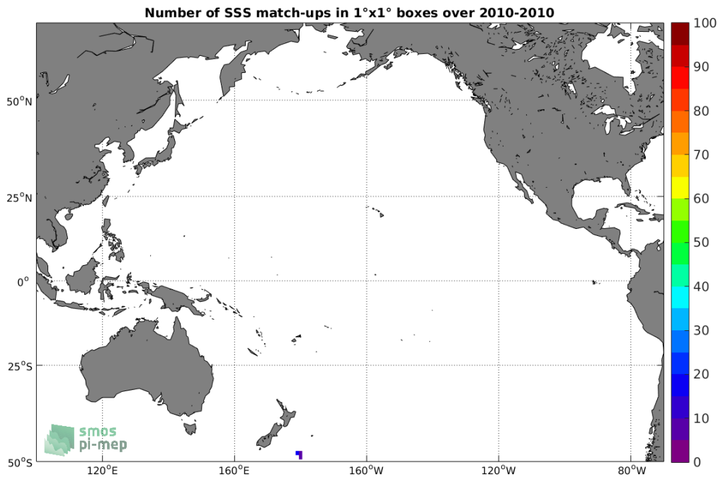
Figure 4: Number of SSS match-ups between TSG (Polarstern) SSS and the SMOS SSS L3 v317 - 10 Days - 25 km (CATDS-CPDC) SSS product for the Pacific Ocean Pi-MEP region over 1°x1° boxes and for the full satellite product period.
