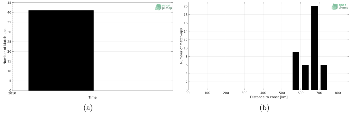
Figure 1: Number of match-ups between TSG-POLARSTERN and SMOS L3 v317 - 10 Days - 25 km (CATDS-CPDC) SSS as a function of time (a) and as function of the distance to coast (b) over the Pacific Ocean Pi-MEP region and for the full satellite product period.
