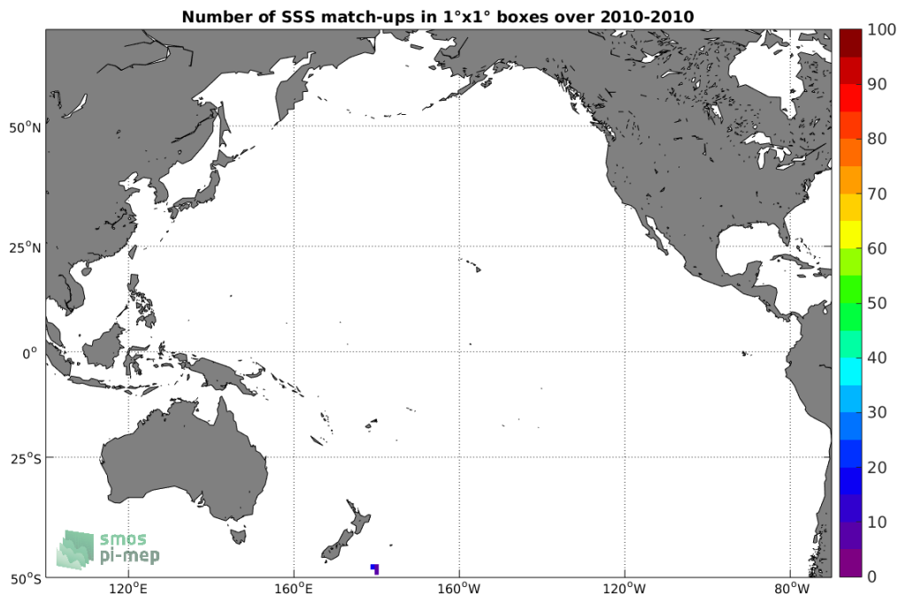
Figure 4: Number of SSS match-ups between TSG-POLARSTERN SSS and the SMOS L3 v317 - 10 Days - 25 km (CATDS-CPDC) SSS product for the Pacific Ocean Pi-MEP region over 1^\circ \times 1^\circ boxes and for the full satellite product period.
