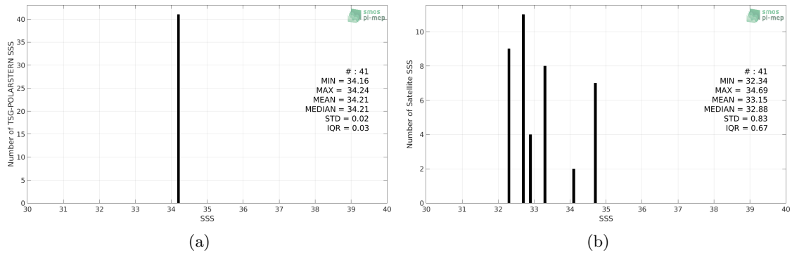
Figure 2: Histograms of SSS from TSG-POLARSTERN (a) and SMOS L3 v317 - 10 Days - 25 km (CATDS-CPDC) (b) considering all match-up pairs per bins of 0.1 over the Pacific Ocean Pi-MEP region and for the full satellite product period.
