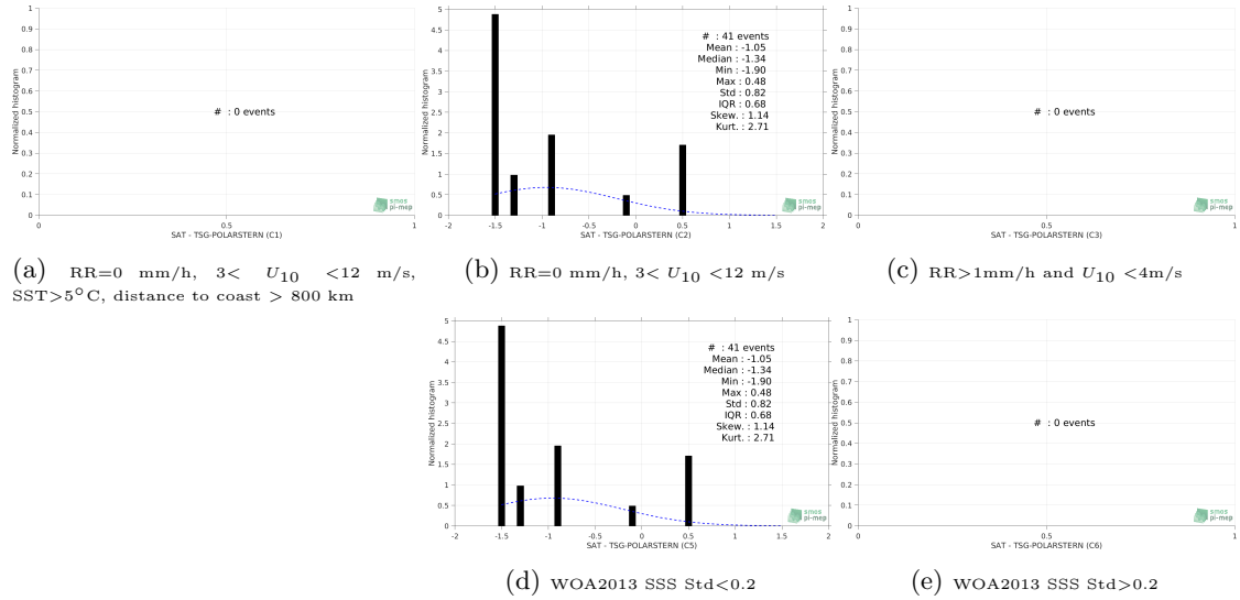
Figure 13: Normalized histogram of \Delta SSS (SMOS L3 v317 - 10 Days - 25 km (CATDS-CPDC) - TSG-POLARSTERN) for 5 different subdatasets corresponding to: RR=0 mm/h, 3 < U_{10} < 12 m/s, SST >5^{\circ} C, distance to coast > 800 km (a), RR=0 mm/h, 3 < U_{10} < 12 m/s (b), RR >1 mm/h and U_{10} < 4 m/s (c), WOA2013 SSS Std <0.2 (d), WOA2013 SSS Std >0.2 (e).
