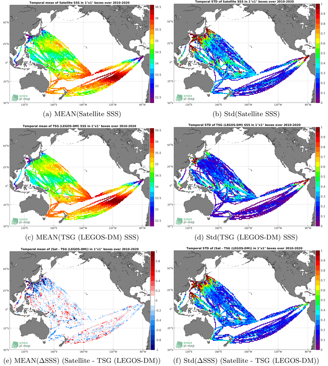
Figure 6: Temporal mean (left) and Std (right) of SSS from SMOS SSS L3 v317 - 10 Days - 25 km (CATDS-CPDC) (top), TSG (LEGOS-DM) (middle), and of \Delta SSS (Satellite - TSG (LEGOS-DM)). Only match-up pairs are used to generate these maps.
