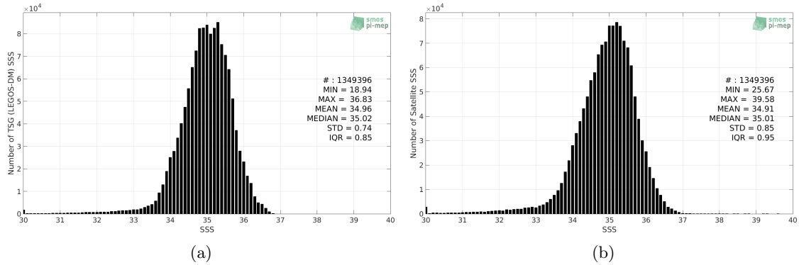
Figure 2: Histograms of SSS from TSG (LEGOS-DM) (a) and SMOS SSS L3 v317 - 10 Days - 25 km (CATDS-CPDC) (b) considering all match-up pairs per bins of 0.1 over the Pacific Ocean Pi-MEP region and for the full satellite product period.
