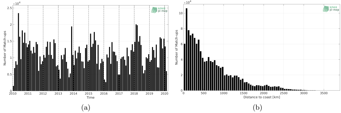
Figure 1: Number of match-ups between TSG (LEGOS-DM) and SMOS SSS L3 v317 - 10 Days - 25 km (CATDS-CPDC) SSS as a function of time (a) and as function of the distance to coast (b) over the Pacific Ocean Pi-MEP region and for the full satellite product period.
