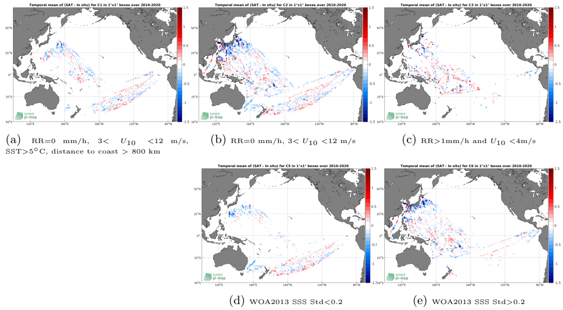
Figure 12: Temporal mean gridded over spatial boxes of size 1^\circ \times 1^\circ of \Delta SSS (SMOS SSS L3 v317 - 10 Days - 25 km (CATDS-CPDC) - TSG (LEGOS-DM)) for 5 different subdatasets corresponding to: RR=0 mm/h, 3 < U_{10} < 12 m/s, SST >5^\circ\text{C} , distance to coast > 800 km (a), RR=0 mm/h, 3 < U_{10} < 12 m/s (b), RR >1 mm/h and U_{10} < 4 m/s (c), WOA2013 SSS Std <0.2 (d), WOA2013 SSS Std >0.2 (e).
