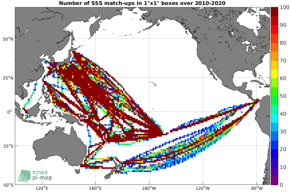
Figure 4: Number of SSS match-ups between TSG (LEGOS-DM) SSS and the SMOS SSS L3 v317 - 10 Days - 25 km (CATDS-CPDC) SSS product for the Pacific Ocean Pi-MEP region over 1^\circ \times 1^\circ boxes and for the full satellite product period.
