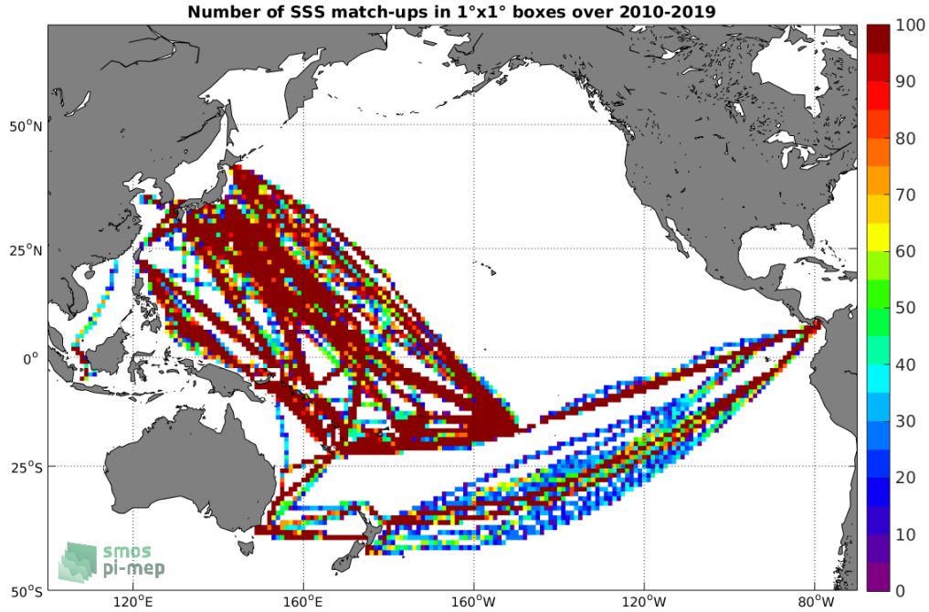
Figure 4: Number of SSS match-ups between TSG (LEGOS-DM) SSS and the SMOS SSS L3 v317 - 10 Days - 25 km (CATDS-CPDC) SSS product for the Pacific Ocean Pi-MEP region over 1°x1° boxes and for the full satellite product period.
