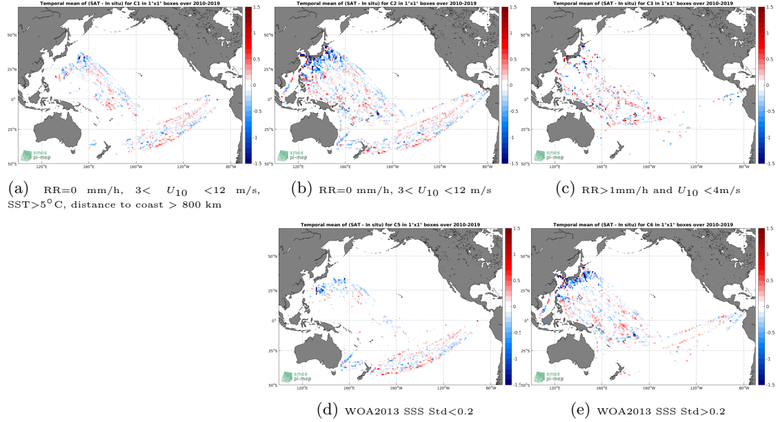
Figure 12: Temporal mean gridded over spatial boxes of size 1^\circ \times 1^\circ of \Delta SSS (SMOS L3 v317 - 10 Days - 25 km (CATDS-CPDC) - TSG-LEGOS-DM) for 5 different subdatasets corresponding to: RR=0 mm/h, 3 < U_{10} < 12 m/s, SST > 5^\circ C , distance to coast > 800 km (a), RR=0 mm/h, 3 < U_{10} < 12 m/s (b), RR > 1 mm/h and U_{10} < 4 m/s (c), WOA2013 SSS Std < 0.2 (d), WOA2013 SSS Std > 0.2 (e).
