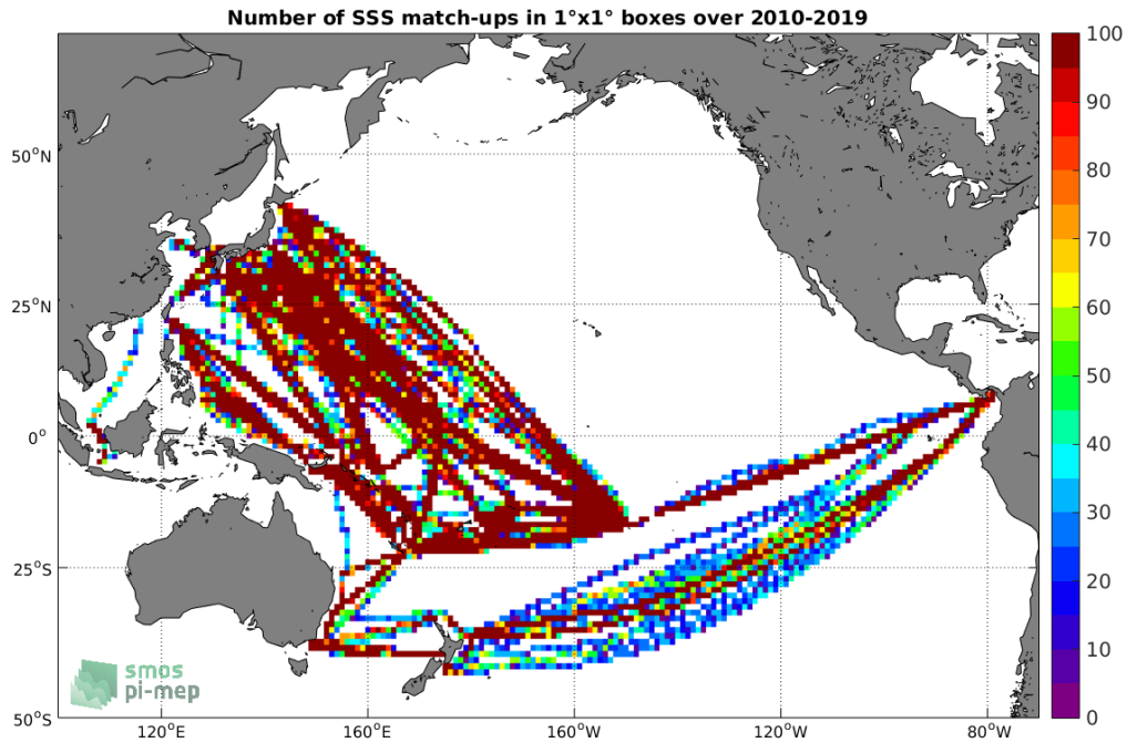
Figure 4: Number of SSS match-ups between TSG-LEGOS-DM SSS and the SMOS L3 v317 - 10 Days - 25 km (CATDS-CPDC) SSS product for the Pacific Ocean Pi-MEP region over 1°x1° boxes and for the full satellite product period.
