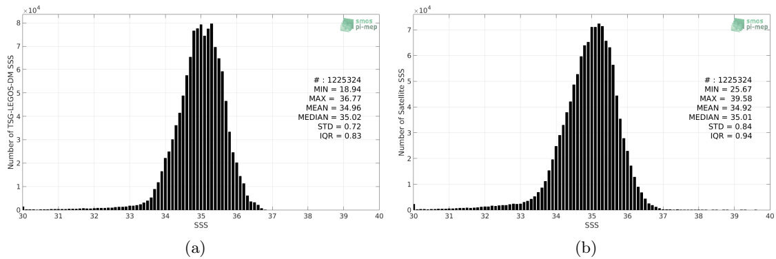
Figure 2: Histograms of SSS from TSG-LEGOS-DM (a) and SMOS L3 v317 - 10 Days - 25 km (CATDS-CPDC) (b) considering all match-up pairs per bins of 0.1 over the Pacific Ocean Pi-MEP region and for the full satellite product period.
