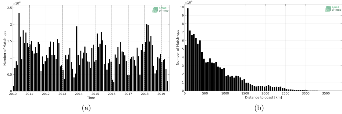
Figure 1: Number of match-ups between TSG-LEGOS-DM and SMOS L3 v317 - 10 Days - 25 km (CATDS-CPDC) SSS as a function of time (a) and as function of the distance to coast (b) over the Pacific Ocean Pi-MEP region and for the full satellite product period.
