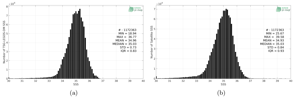
Figure 2: Histograms of SSS from TSG-LEGOS-DM (a) and SMOS-L3-CATDS-CPDC-V317-10DAYS-25KM (b) considering all match-up pairs per bins of 0.1 over the Pacific Ocean Pi-MEP region and for the full satellite product period.
