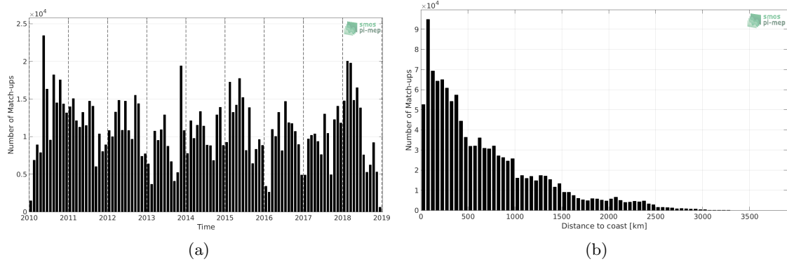
Figure 1: Number of match-ups between TSG-LEGOS-DM and SMOS-L3-CATDS-CPDC-V317-10DAYS-25KM SSS as a function of time (a) and as function of the distance to coast (b) over the Pacific Ocean Pi-MEP region and for the full satellite product period.
