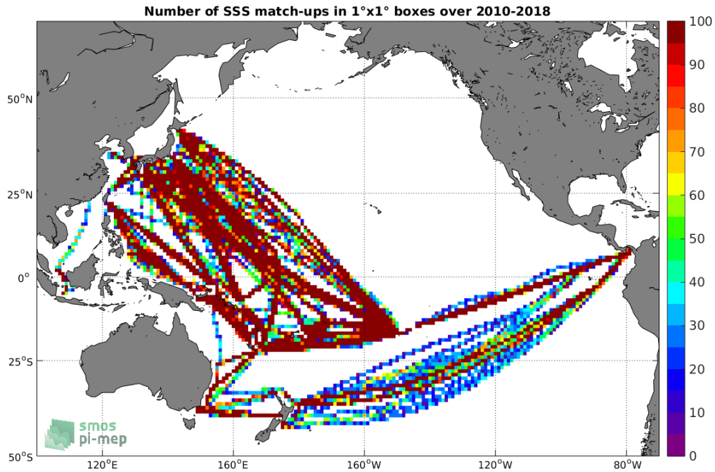
Figure 4: Number of SSS match-ups between TSG-LEGOS-DM SSS and the SMOS-L3-CATDS-CPDC-V317-10DAYS-25KM SSS product for the Pacific Ocean Pi-MEP region over 1°x1° boxes and for the full satellite product period.
