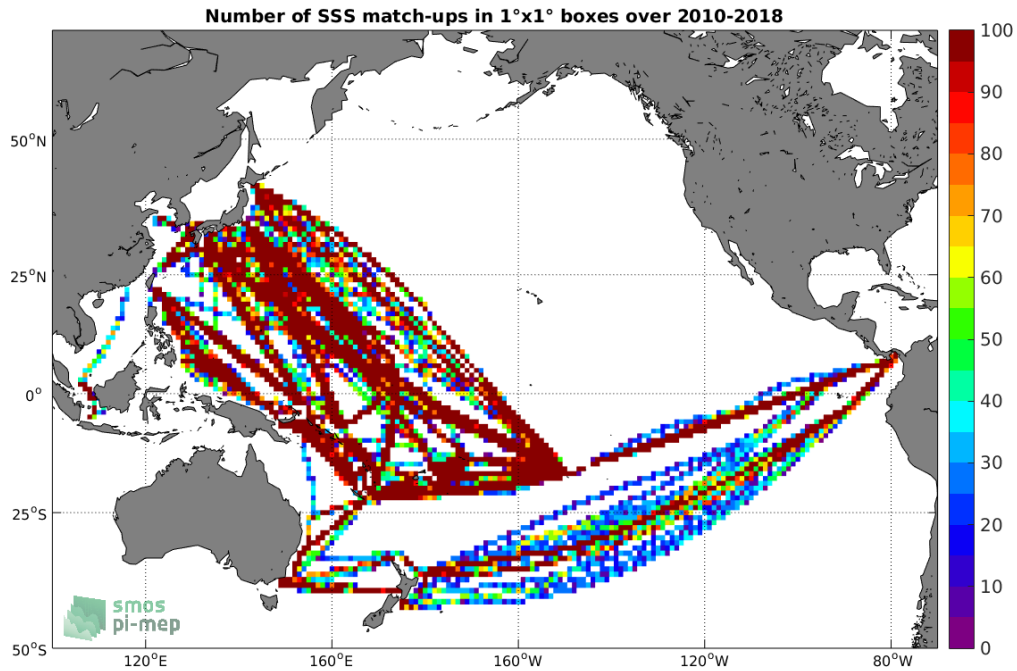
Figure 4: Number of SSS match-ups between TSG-LEGOS-DM SSS and the SMOS-L3-CATDS-CPDC-V317-10DAYS-25KM SSS product for the Pacific Ocean Pi-MEP region over 1^\circ \times 1^\circ boxes and for the full satellite product period.
